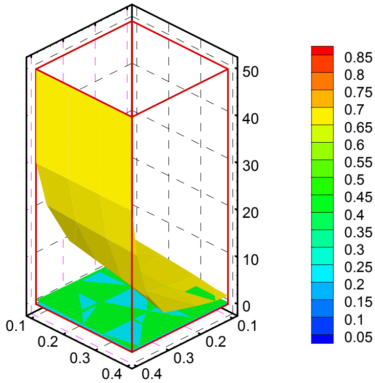
Fig.3-1 the stress singular index \lambda varying with the materials parameter \frac{\mu_2}{\mu_1} , \nu_1 , \nu_2
