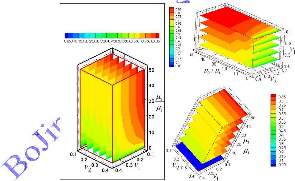
Fig.3-2. the stress singular index \lambda varying with the materials parameter \frac{\mu_2}{\mu_1} , \nu_1 , \nu_2
