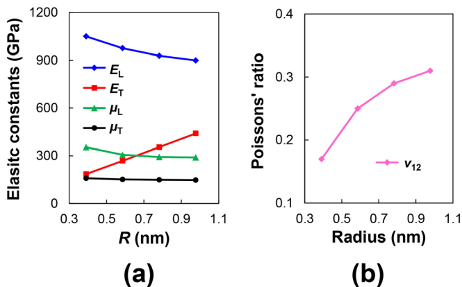
FIG. 3. The predicted (a) elastic constants and (b) the Poisson's ratio of CNTs from MS simulations.
