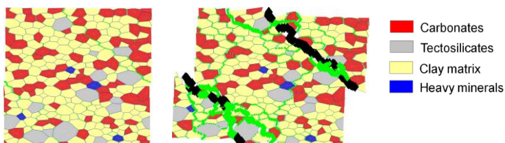
Microstructure deformation
