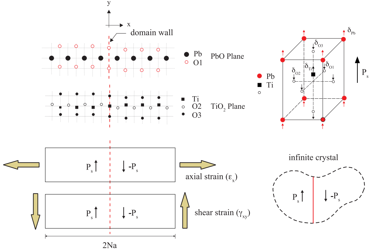
Figure 2.1: Reference configuration for a Ti-centered 180^\circ domain wall in PbO and \text{TiO}_2 planes. Note that cores and shells on the domain wall have no relative shifts and cores and shells on the left and right sides of the wall have opposite relative shifts. a and N are lattice parameter and size of the simulation box, respectively.
