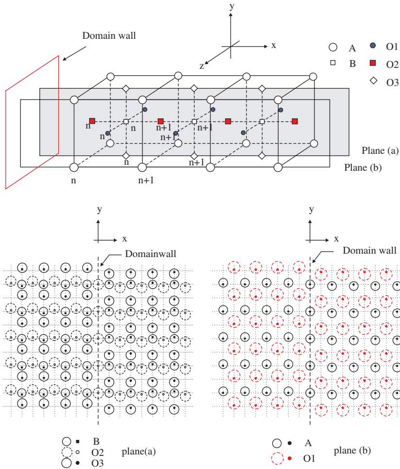
Figure 4. Reference configuration for an A-centred 180^\circ domain wall shown in the two planes (a) and (b). Note that the reference configuration is invariant under the transformation x \rightarrow -x, y \rightarrow -y, z \rightarrow z (or -z ).
