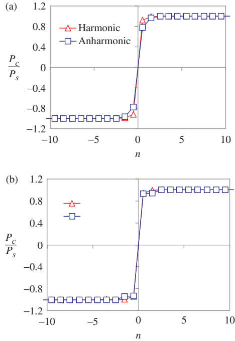
Figure 9. Harmonic and anharmonic polarization distributions for (a) Pb and (b) Ti-centred 180^\circ domain walls.
