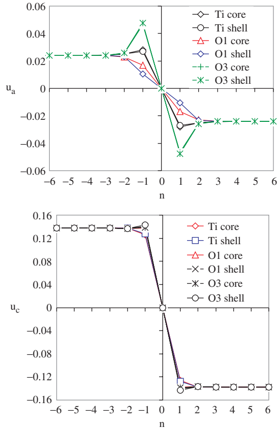
Figure 8. Anharmonic displacements of Ti, O1 and O3 cores and shells for a Ti-centred 180° domain wall.
