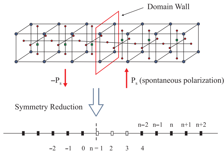
Figure 3. Reference configuration used in analysis of a 180° domain wall.
