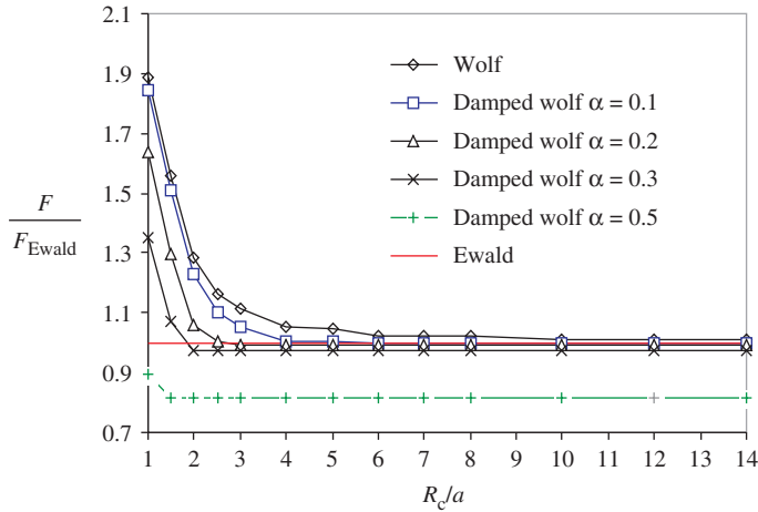
Figure 16. Pb core force in tetragonal direction in PbTiO_3 .
