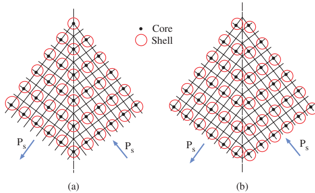
Figure 10. Reference configuration of (a) A cores and shells and (b) O2 cores and shells for a ABO1-centred nominal 90^\circ domain wall.
