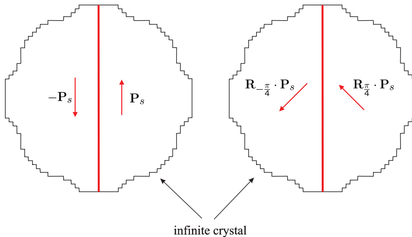
Figure 2. Single 180° and 90° domain walls in infinite crystals with the bulk far-field conditions. P_s is the spontaneous polarization vector and R_{-\pi/4} and R_{\pi/4} are rotation matrices.
