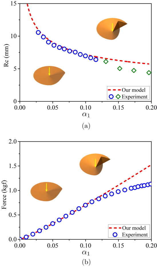
FIG. 5. Comparison of our model with the experimental data reported in Ref. [5] for the purely mechanical problem of a crumpling sheet. (a) The dimensionless tip deflection \alpha_1 = d/R vs the radius of core part R_c = R\alpha_2 of a crumpling sheet. (b) The dimensionless tip deflection \alpha_1 vs the vertical force F applied on the center of a thin sheet of steel. The vertical force is approximately linear with the tip deflection for small deformation. This linear relation is analogous to the relation between the center load and the maximum deflection of a simply supported beam. Note the notation difference that, in Ref. [5], the tip deflection (horizontal axis) is denoted by \epsilon = d/R .
