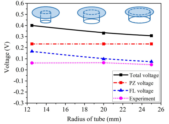
FIG. 6. Comparisons of the generated voltage of a crumpling sheet predicted by our model with the experimental data by Kodali et al. [37] with different supporting hoops. In our model, we consider both the contributions of piezoelectricity and flexoelectricity while the experiments can only calibrate the total voltage on the upper and lower surfaces of a crumpling sheet.
