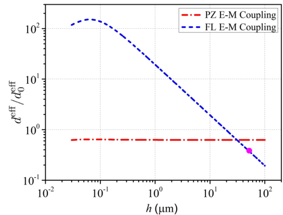
FIG. 4. Flexoelectric and piezoelectric effects vs the sheet thickness h . The effective effect (electromechanical coupling) is defined as d^{\text{eff}} = Q/F , and is normalized by d_0^{\text{eff}} = 652 pC/N that is calculated by the geometrical and material parameters in Fig. 3 at tip depth d = 4 mm. The experimental data (solid circle, d^{\text{eff}}/d_0^{\text{eff}} = 0.38 ) of the effective effect of a thin sheet with thickness h = 52 \mu\text{m} is also plotted for comparison between different thicknesses. The reported piezoelectric coefficient of barium titanate is around d^{\text{BaTiO}_3} = 78 pC/N.
