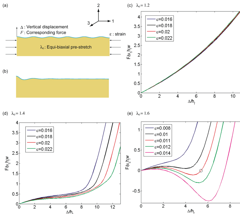
Figure 4. Finite element simulation results. a) Simulation showing wrinkles under an equi-biaxial strain of \varepsilon = 0.011 and a pre-stretch of \lambda_0 = 1.6 in the substrate. b) Simulation showing the large amplitude ridge state under the same loading condition as in (a). In (a) and (b), the blue line represents the thin film, and the yellow–brown area represents the substrate. c–e) F – \Delta curves are obtained for various fixed strains for an equi-biaxial pre-stretch of \lambda_0 = 1.2 (c), 1.4 (d), and 1.6 (e) with \mu_f/\mu_s = 2000 and (h_f + h_s)/h_f = 50 .
