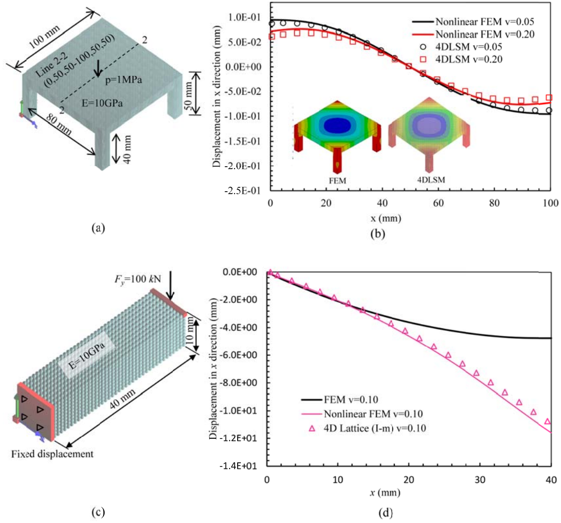
Figure 6. Elastic problems solved by the 4D lattice spring model: (a) computational model of a table's deformation problem; (b) FEM and the 4D lattice spring model solutions with different Poisson's ratios; (c) computation of the nonlinear beam bending problem; and (d) nonlinear beam bending problem solved by linear FEM, nonlinear FEM and the 4D lattice spring model.
