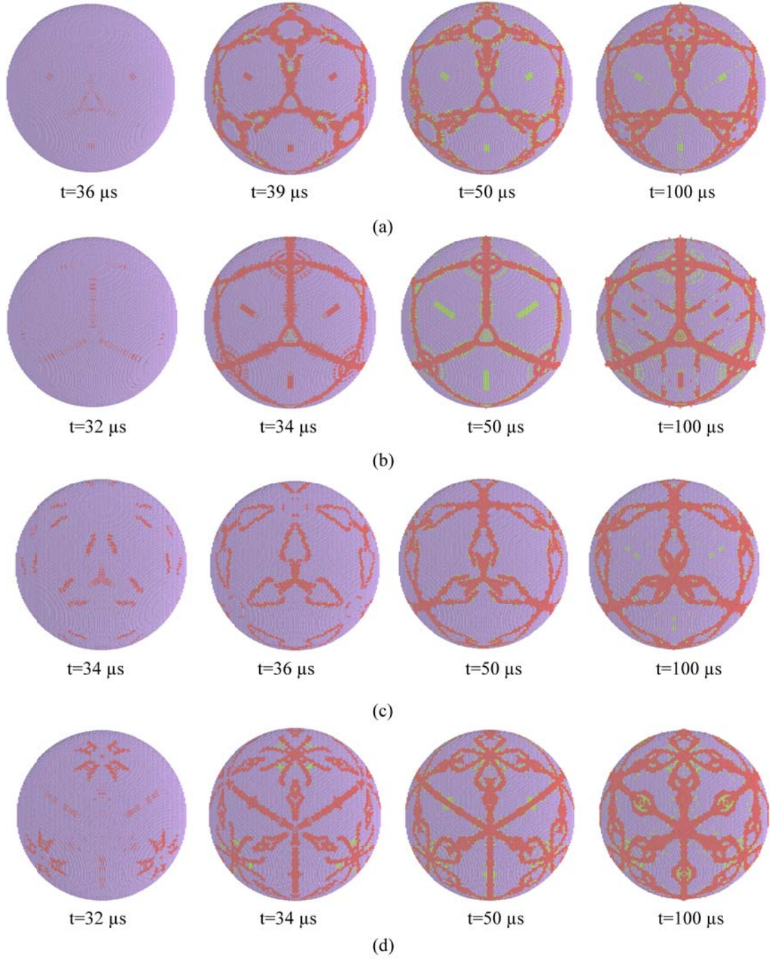
Figure 8. Dynamic fracturing process of a hollow sphere under blasting loading with different Poisson's ratios and spring strengths (blue represents to the original solid, red indicates failure with particle opening, and green represents failure with particle closure), (a) \nu = 0.05 , u_n^* = 3.5 \times 10^{-3} mm, (b) \nu = 0.05 , u_n^* = 3.0 \times 10^{-3} mm, (c) \nu = 0.23 , u_n^* = 3.5 \times 10^{-3} mm, and (d) \nu = 0.23 , u_n^* = 3.0 \times 10^{-3} mm.
