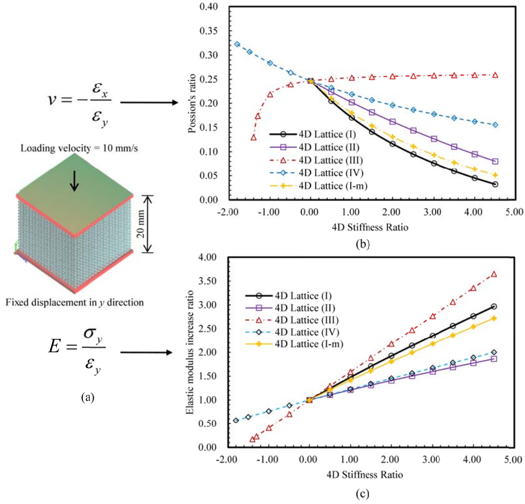
Figure 2. Relationship between the 4D stiffness ratio \lambda^{4D} and elastic constants obtained from numerical simulation of a uniaxial compression test: (a) computational model (strain and stress are calculated from average force/displacement values of the corresponding cubic specimen surfaces), (b) relationship between \lambda^{4D} and the Poisson's ratio, and (c) relationship between \lambda^{4D} and the elastic modulus increase ratio.
