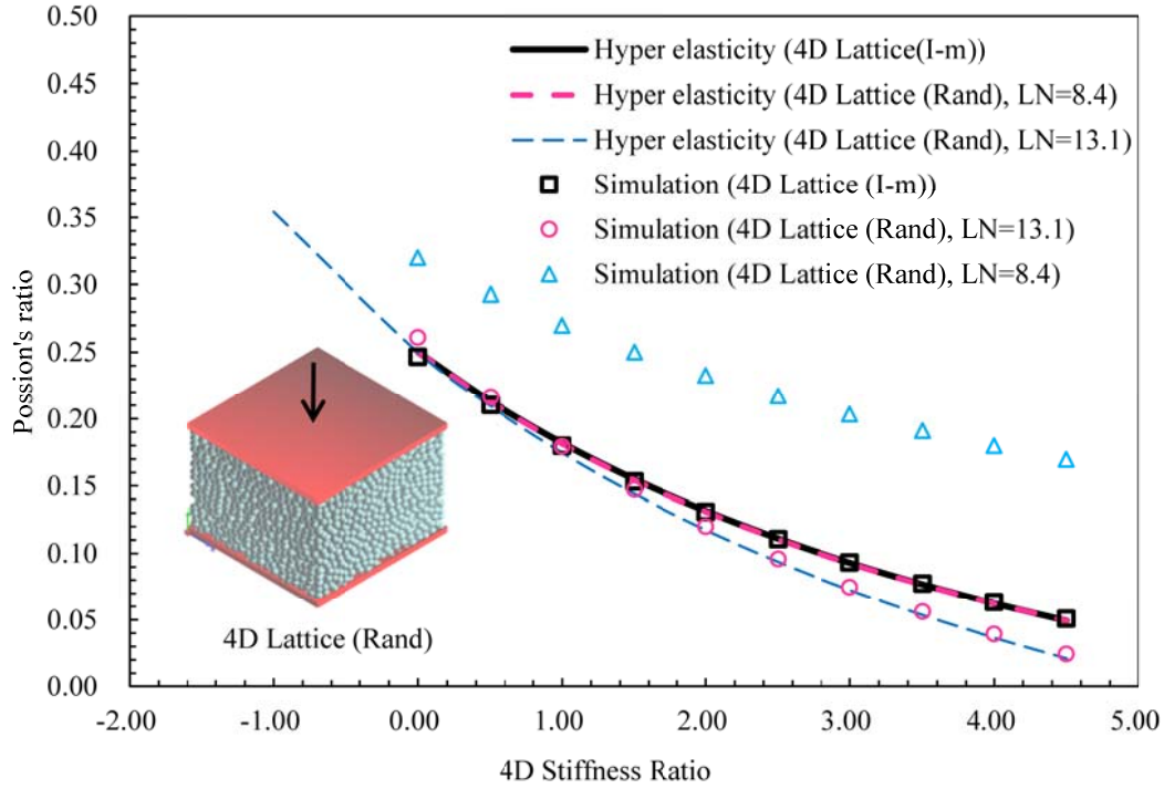
Figure 3. Poisson's ratios predicted by hyperelasticity analysis and by numerical simulation using the 4D lattice spring model.
