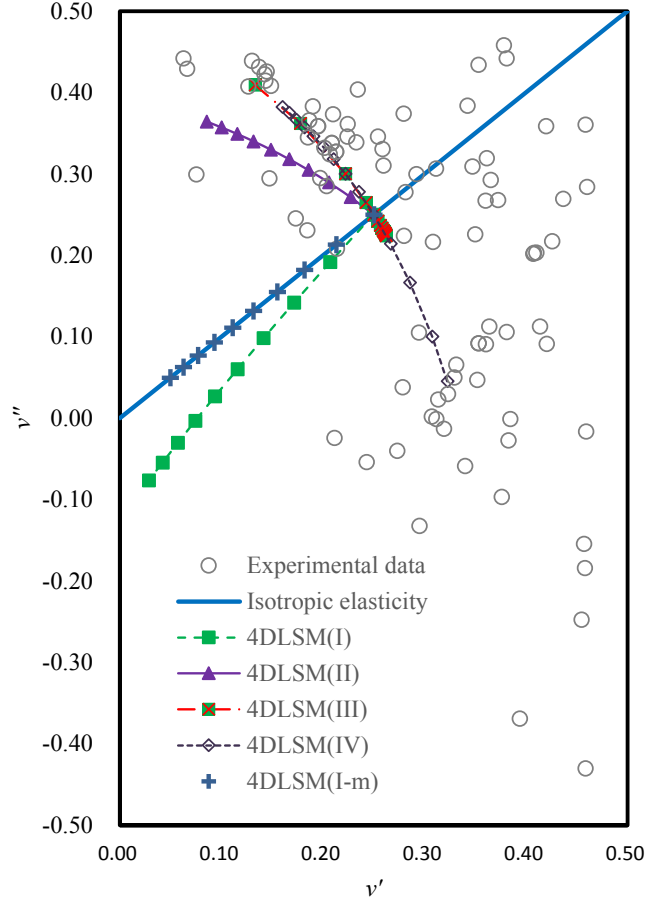
Figure 4. Poisson's ratios of cubic lattice models calculated from hyperelasticity analysis ( k_\alpha \in [-4, 5] , k_\beta \in [-4, 5] , and k_\gamma \in [-4, 5] ); experimental data for cubic crystals [18] are also shown.
