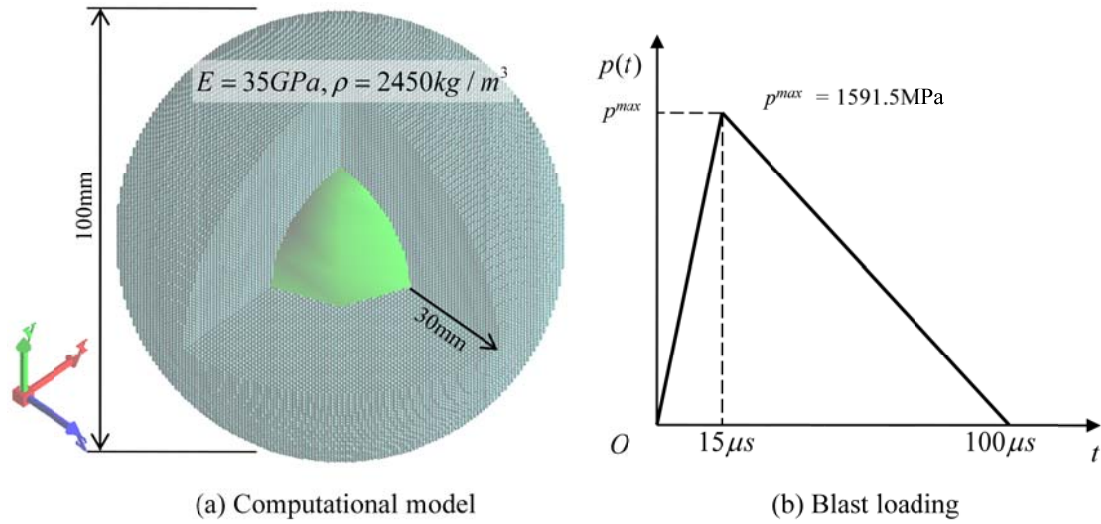
Figure 7. Dynamic fracturing of a hollow sphere under blast loading: (a) computational model and boundary condition and (b) blasting represented as a triangle pressure loading.
