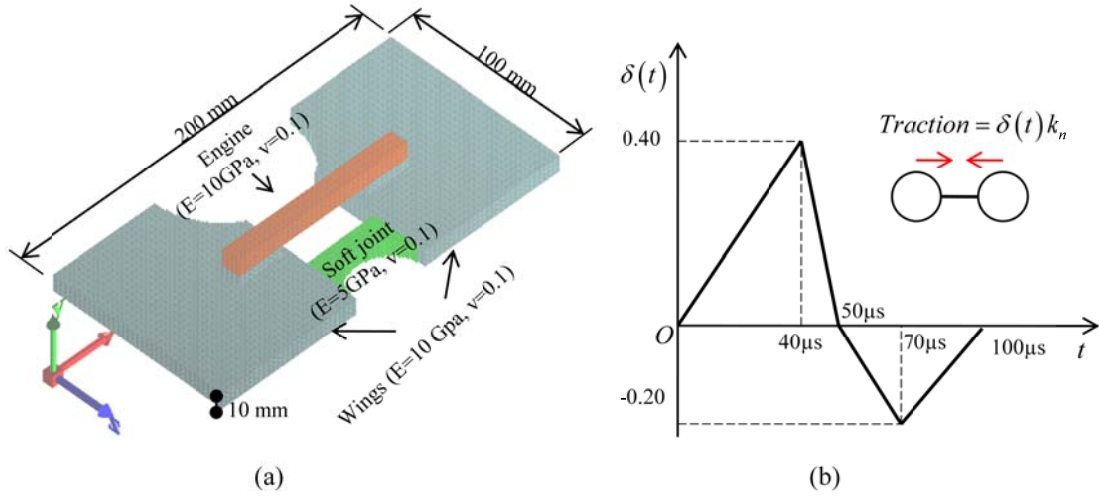
Figure 9. Dynamic motion of a soft robot: (a) computational model and (b) input pulse for the engine material.
