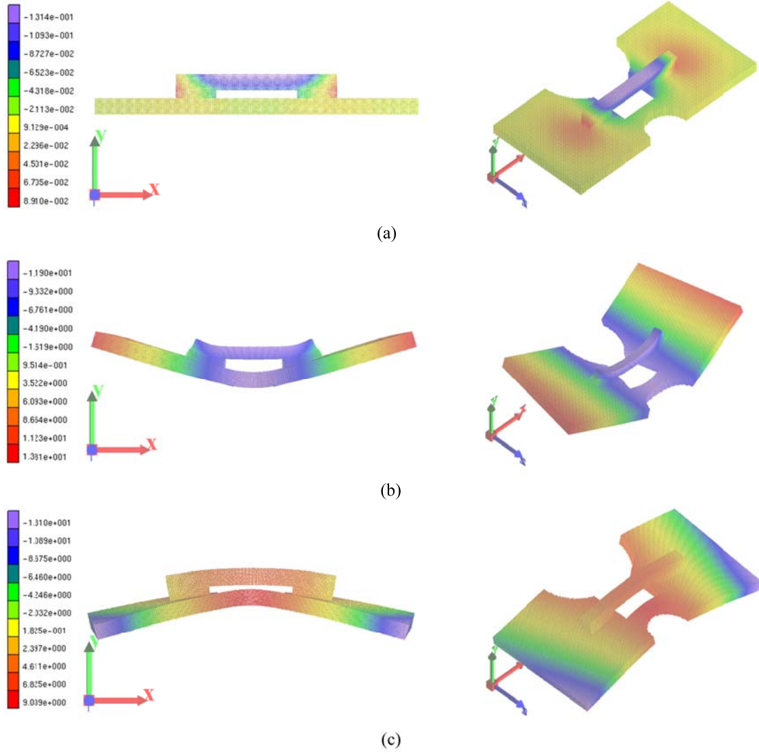
Figure 10. Dynamic deforming of the soft robot predicted by the 4D lattice spring model (contour map of displacement in the y -direction): (a) t = 1 \mu s , (b) t = 40 \mu s , and (c) t = 90 \mu s .
