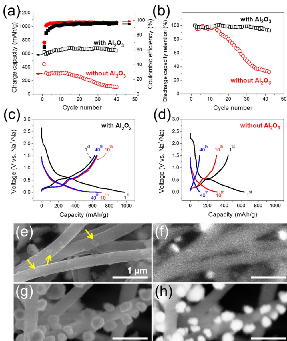
Figure 4. Results of coin-cell electrochemical tests and ex situ SEM. (a–d) Comparison of battery performance using SnNPs@CNF anodes with and without an ALD-Al 2 O 3 coating in half-cell for NIBs: (a) Discharge/charge cycle performance and Coulombic efficiency. (b) Discharge capacity retention. (c,d) Voltage profiles of the 1st, 10th, and 40th cycle. (e–h) Ex situ SEM images for the anodes without (e,f) and with (g,h) ALD-Al 2 O 3 coating disassembled from the coin-cell battery after 40 cycles. The SEM images in (e,g) are recorded with the secondary electron (SE) detector, and those in (f,h) are recorded with the backscattered electron (BSE) detector. The yellow arrows in (e) indicate the traces of fallen SnNPs left on carbon fibers. The scale bars in (e–h) are 1 μm.
