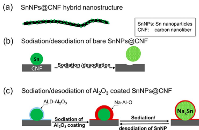
Figure 1. Schematic of the hybrid anode nanostructures and their corresponding sodiation processes. (a) The hybrid nanostructure SnNPs@CNF. (b) During sodiation/desodiation, a bare SnNP debonds from the carbon nanofiber substrate. (c) For the ALD- \text{Al}_2\text{O}_3 coated SnNPs@CNF, the ALD- \text{Al}_2\text{O}_3 coating is first uniformly converted to a Na-Al-O layer, followed by the reversible sodiation/desodiation of the SnNP core. Note that the Na-Al-O layer deforms to accommodate the swelling and shrinking of the SnNP core, maintaining the anode structural integrity.
