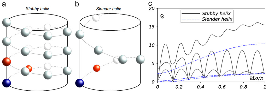
Fig. 16. Energy transport in helices with different aspect ratios using model interatomic potentials. The red atoms are the near-neighbors of the blue atom in real-space. In the slender helix, there is no long-range interaction and it behaves like a 1D chain. The stubby helix has long-range interaction and has prominent wiggles in the phonon spectrum. (For interpretation of the references to color in this figure caption, the reader is referred to the web version of this article.)
