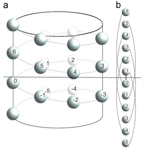
Fig. 15. A schematic of the geometric model for energy transport (a) in real space, (b) in Objective Space. The energy flow to be analyzed takes place across the bold dashed line, i.e. how much energy do subunits 0, −1, −2, ... transfer to the subunits 1, 2, 3, ... The subunits can correspond to individual atoms or sets of atoms.
