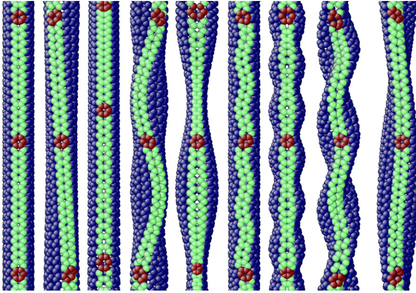
Fig. 6. An assortment of phonon modes at finite wavevectors. First figure is the reference state. The colors of the atoms have no significance and are only to enable easy visualization. (For interpretation of the references to color in this figure caption, the reader is referred to the web version of this article.)
