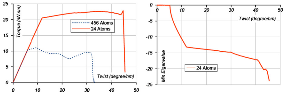
Fig. 11. Left: twisting moment vs. twist angle using atomistics. Right: lowest eigenvalue vs. twist angle for the smaller unit cell.
