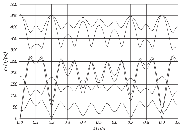
Fig. 13. Dispersion curves of a (11,9) carbon nanotube. FD contains two atoms.
