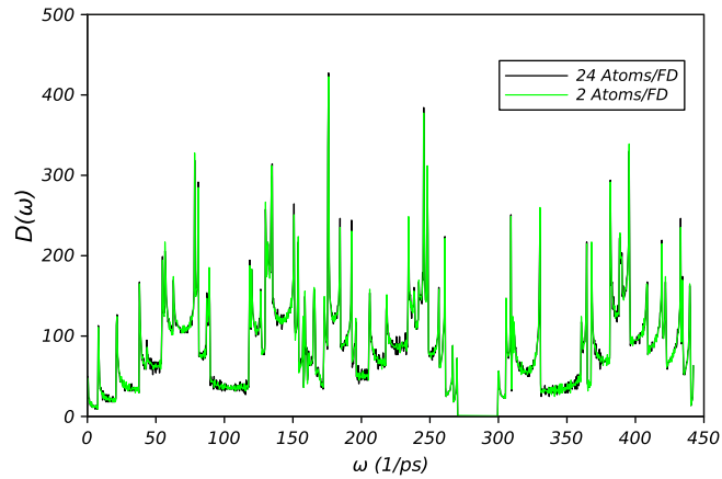
Fig. 7. Density of states of a (6,6) nanotube.
