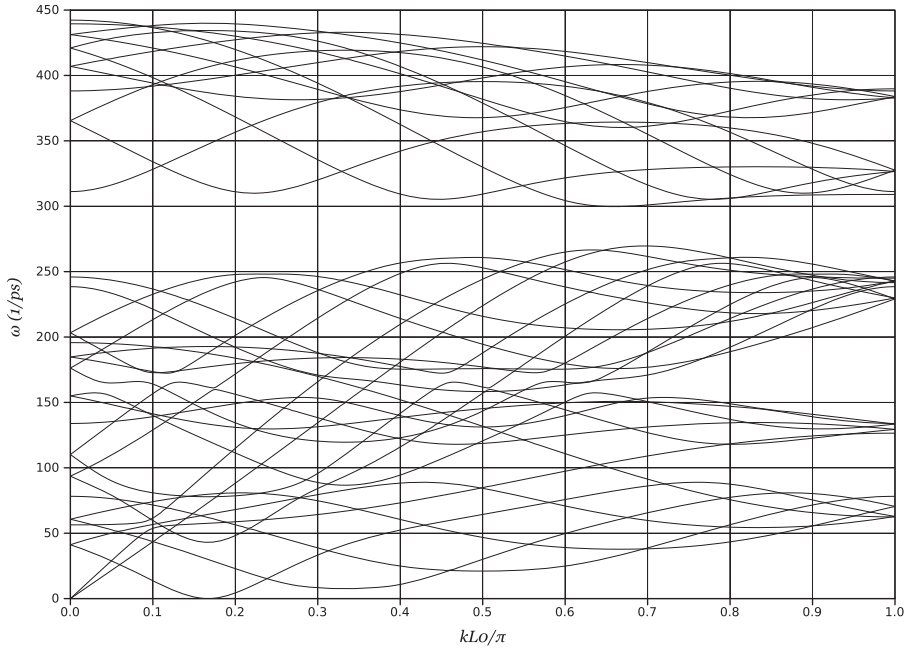
Fig. 2. Dispersion curves of a (6,6) carbon nanotubes using Choice 3. The wavevector is normalized by the length of the translation vector 0.123 nm in g_2 . The band-folding shows that our unit cell still has unused symmetries.
