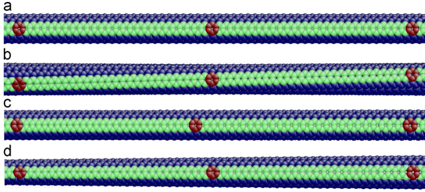
Fig. 4. Phonon modes at k_1 \approx 0 and k_2 = 0 using Choice 4. (a) The undeformed reference nanotube. The colors of the atoms are only to enable visualization of the deformation. (b) The lowest branch corresponding to twisting. (c) The next-to-lowest branch corresponding to axial elongation. (d) The third-from-lowest branch corresponding to a change in radius. In each of these deformations, the cross-section remains circular. (For interpretation of the references to color in this figure caption, the reader is referred to the web version of this article.)
