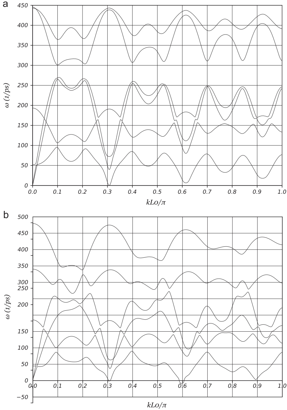
Fig. 14. Dispersion curves of a (7,6) carbon nanotube. FD contains two atoms. (a) Relaxed nanotube. (b) Compressed and twisted nanotube.
