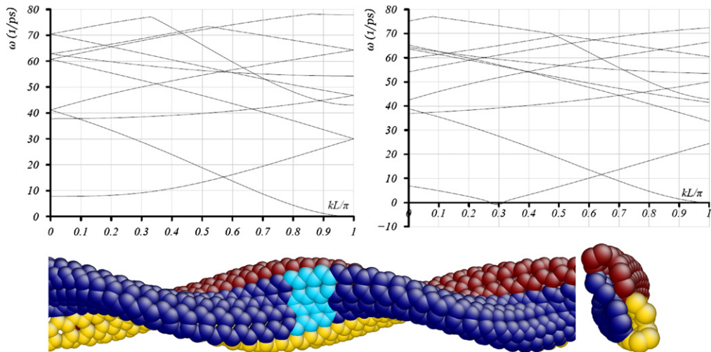
Fig. 12. Phonon stability analysis. Top left: ten lowest modes for the untwisted nanotube. Top right: ten lowest modes just after the lowest eigenvalues becomes negative. The value of the discrete wavevector is 2/3\pi . The twist angle at this state is about 5^\circ/\text{nm} . The mode going to 0 in both plots corresponds to long-wavelength bending. Bottom: the eigenmode corresponding to the zero eigenvalue. This shows the deformation predicted by phonon analysis to have zero energy. Light blue atoms denote a single unit cell. The colors are only to aid visualization. (For interpretation of the references to color in this figure caption, the reader is referred to the web version of this article.)
