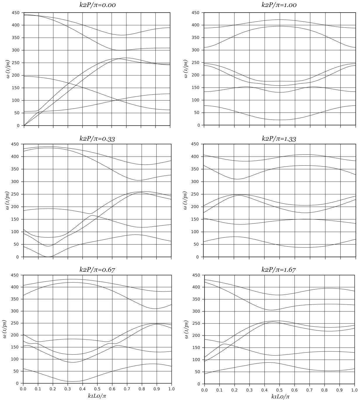
Fig. 3. Dispersion curves of a (6,6) carbon nanotube using Choice 4 with two atoms in the unit cell. k_1 is the component of the wavevector in the continuous direction and normalized by 0.123 nm, and k_2 is the component in the discrete direction and normalized by the approximate perimeter P .
