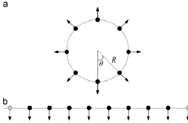
Fig. 9. A long-wavelength mode that corresponds to uniform expansion [mode] and therefore finite energy: (a) A schematic projection, viewed along the axis, of atomic positions and displacements in real space. All displacements are radial. (b) In Objective Space, all atoms displace uniformly, i.e. long wavelength.
