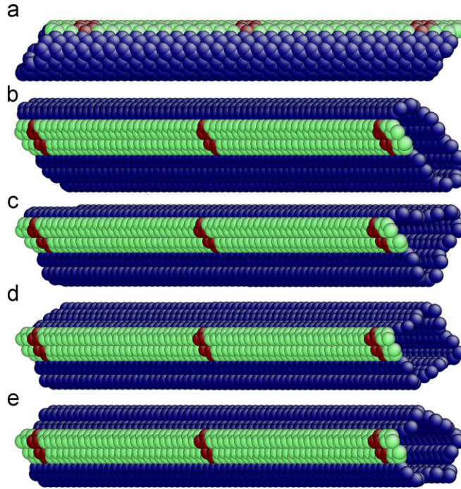
Fig. 5. Some long-wavelength modes at finite k_1 and k_2 using Choice 4 (Fig. 3). The symmetry of the cross-section corresponds to the value of the discrete component of the wavevector. (a) Mode from second branch at k_1 L_0 / \pi = 1/6 and k_2 P / \pi = 1/3 , similar to warping. (b) Mode from first branch at L_0 k_1 / \pi = 1/3 and P k_2 / \pi = 2/3 . (c) Mode from first branch at k_1 L_0 / \pi = 1/2 and P k_2 / \pi = 1 . (d) Mode from first branch at L_0 k_1 / \pi = 2/3 and P k_2 / \pi = 4/3 . (e) Mode from first branch at L_0 k_1 / \pi = 5/6 and P k_2 / \pi = 5/3 .
