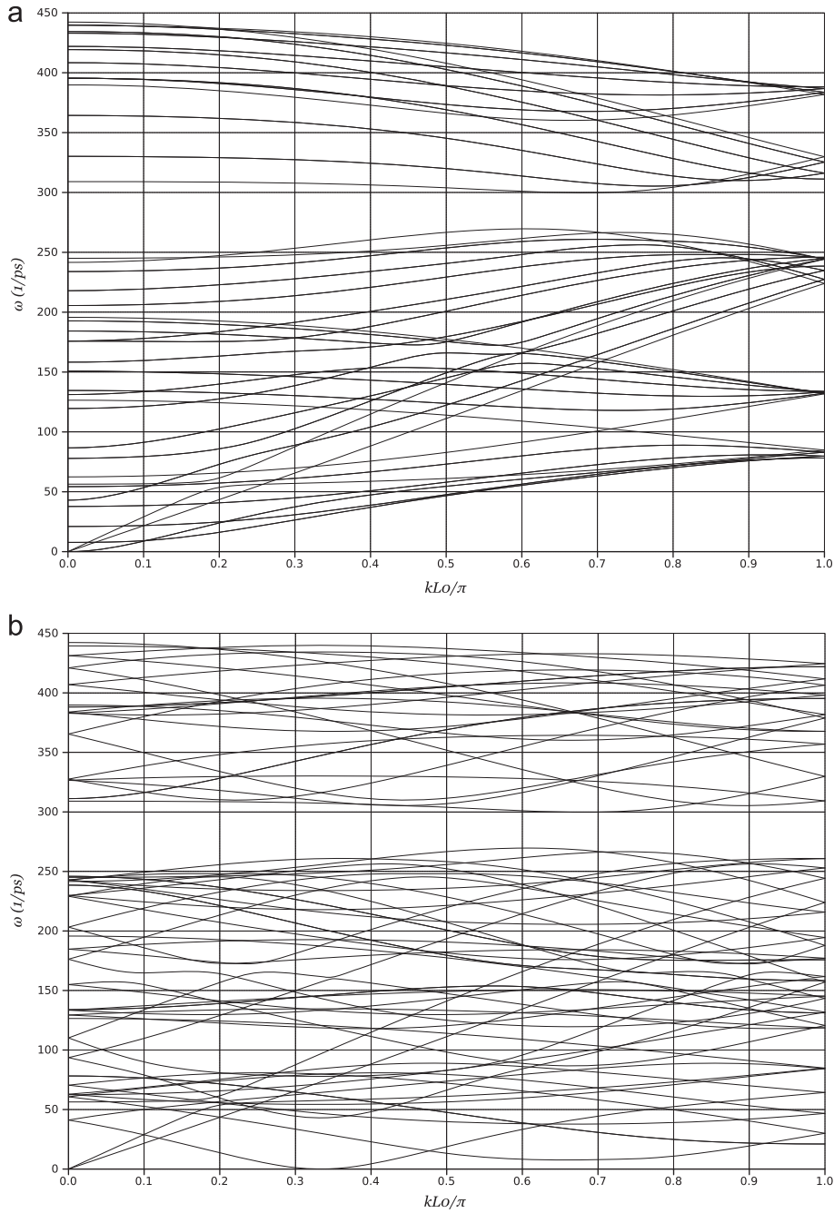
Fig. 1. Dispersion curves of a (6,6) carbon nanotube for (a) Choice 1 and (b) Choice 2. The wavevector is normalized by the length of the translation vector 0.246 nm in g_2 . The large number of phonon curves that have equal and opposite slopes at the right edge of the plots (i.e. “folded over”) are a signature of the large unit cell.
