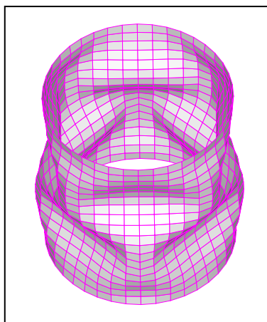
Compression of a (40, 40) CNT
