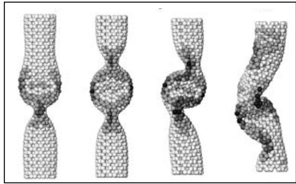
Compression of a (7, 7) CNT (Left) and the corresponding molecular dynamics simulation result by Yakobson et al. (Right, PRL, Vol.76, 1996, 2511-2514)
