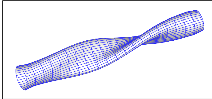
Torsion of a (7, 7) CNT
