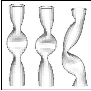
Compression of a (7, 7) CNT (Left) and the corresponding molecular dynamics simulation result by Yakobson et al. (Right, PRL, Vol.76, 1996, 2511-2514)
