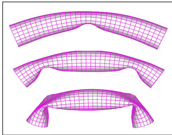
Bending deformation of a (7, 7) CNT with increasing bending angle
