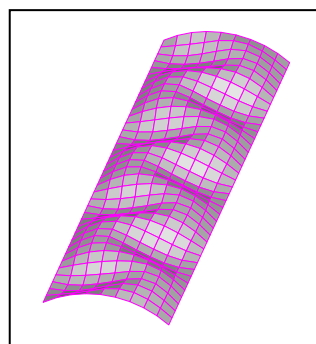
Buckling of a graphene sheet under Bi-axial compression
