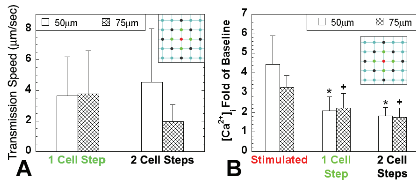
Figure 9 : A) Transmission speed of calcium signal from the indented bone cell to bone cells 1 cell step and 2 cell steps away, in bone cell networks with separation distances of 50 \mu\text{m} or 75 \mu\text{m} . Inset: red = indented cell, green = 1 cell step away, black = 2 cell steps away. There is no significant change in transmission speed regardless of the number of cell steps or separation distances. B) Magnitude of the peak calcium response with each progressive cell step expressed as a fold increase over baseline calcium measurements. There is a significant decrease in calcium response between the indented cell and cells 1 or 2 steps away. * p \leq 0.001 with stimulated cell in 50 \mu\text{m} separation distance network; + p \leq 0.01 with stimulated cell in 75 \mu\text{m} separation distance network. There is no significant difference between the response magnitudes of cells 1 step or 2 steps away for either separation distance. Results are expressed as means \pm standard deviations.
