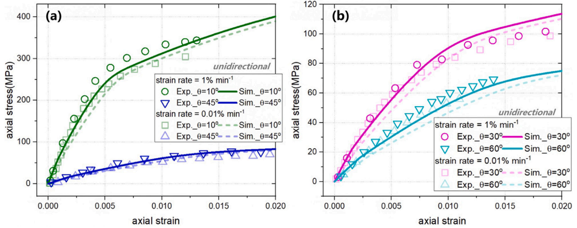
Fig. 7. Off-axis stress-strain curves of single-ply unidirectional composites lamina at different strain rates, the experiment (Masuko and Kawai, 2004) are shown for comparison: (a) \theta = 10^\circ and \theta = 45^\circ , (b) \theta = 30^\circ and \theta = 60^\circ .
