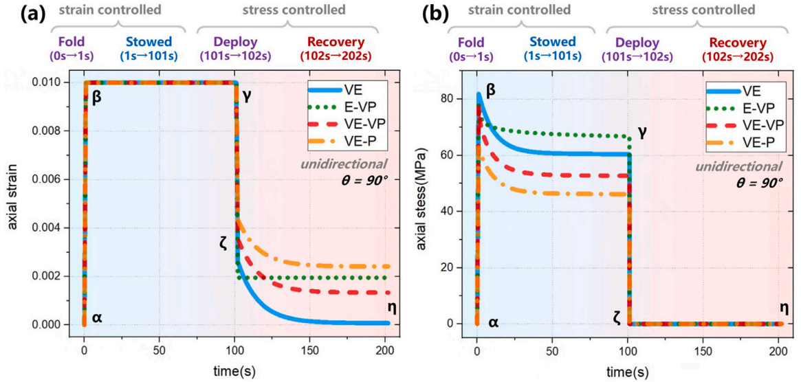
Fig. 10. Relaxation and recovery response of single-ply unidirectional composites lamina based on viscoelastic-viscoplastic (VE-VP) model, the viscoelastic (VE) model, elastic-viscoplastic (E-VP) model and viscoelastic-plastic (VE-P) model responses are shown for comparison: (a) strain-time curves, (b) stress-time curves.
