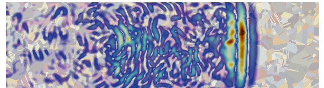
DGFE modeling of ultrasonic wave propagation in real polycrystal - PhD works of A. Talatizi [1].
