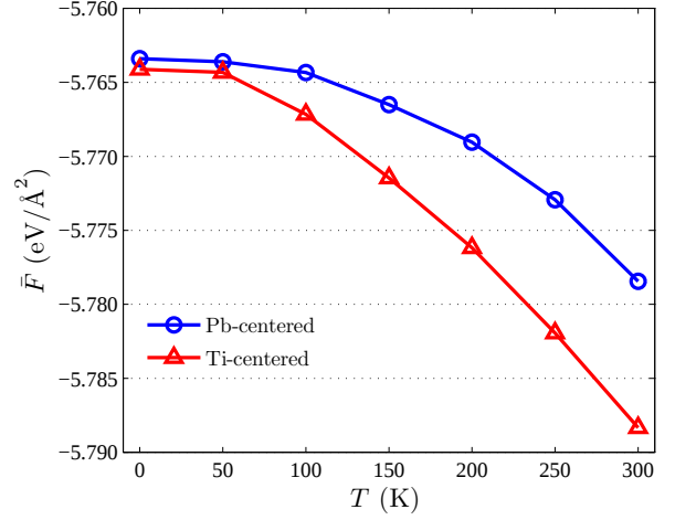
Fig. 4: Free energy of the domain walls as a function of temperature.
