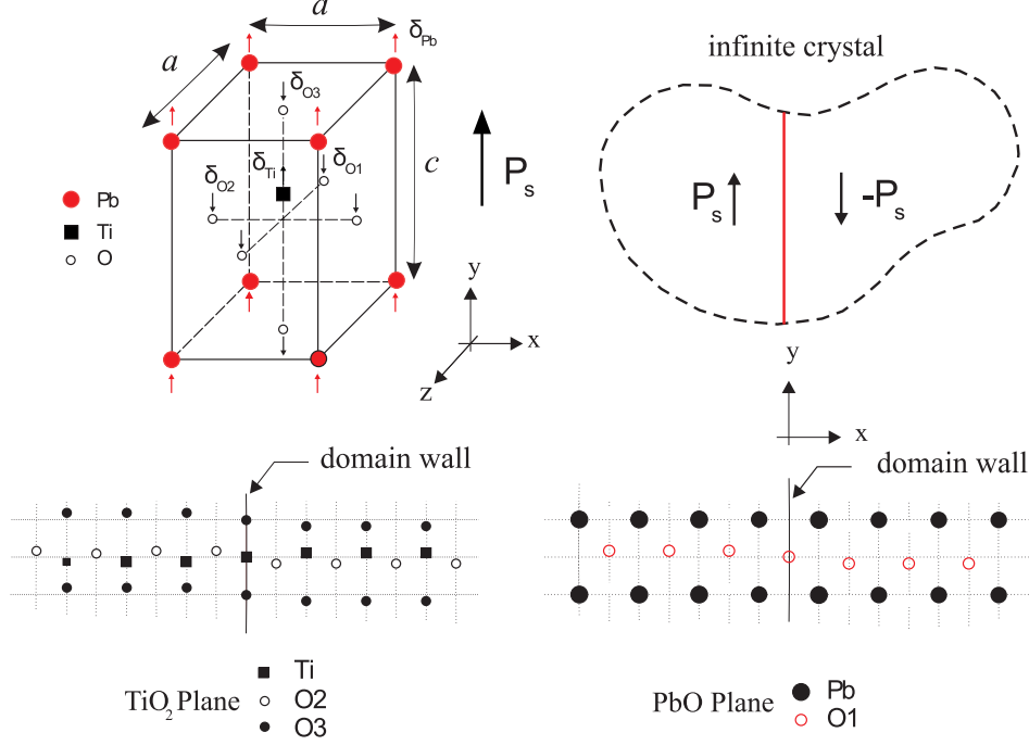
Fig. 1: Reference configuration of a Ti-centered 180^\circ domain wall shown in both the \text{TiO}_2 and \text{PbO} planes. Note that cores and shells on the domain wall have no relative shifts and cores and shells on the left and right sides of the wall have opposite relative shifts.
