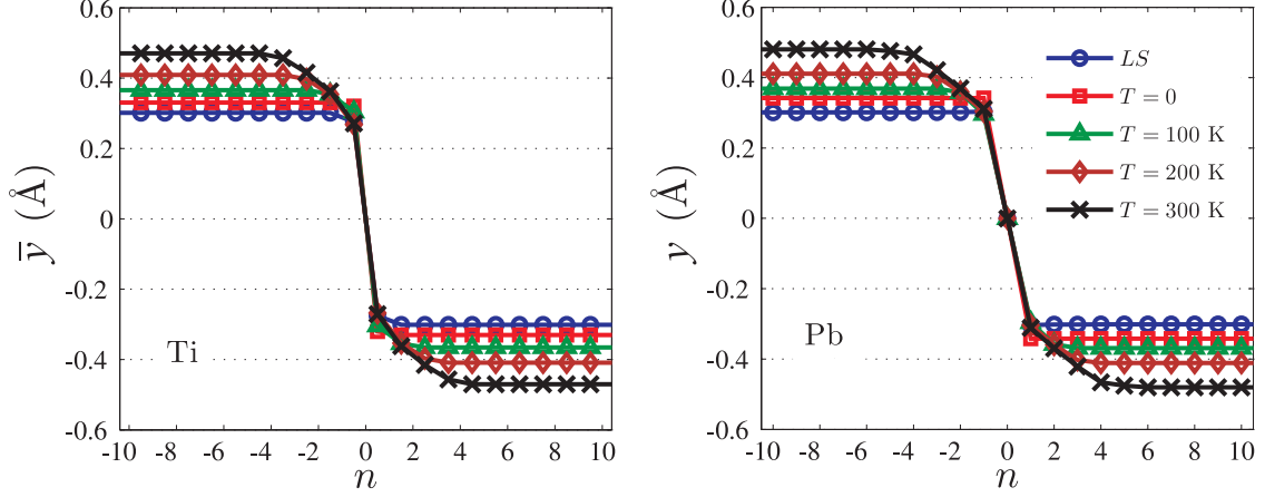
Fig. 2: The y-coordinates of Pb and Ti cores in the Pb-centered 180^\circ domain wall as a function of temperature. LS denotes the lattice statics solution.
