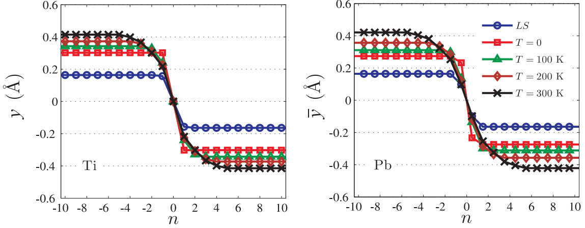
Fig. 3: The y-coordinates of Pb and Ti cores in the Ti-centered 180^\circ domain wall as a function of temperature. LS denotes the lattice statics solution.
