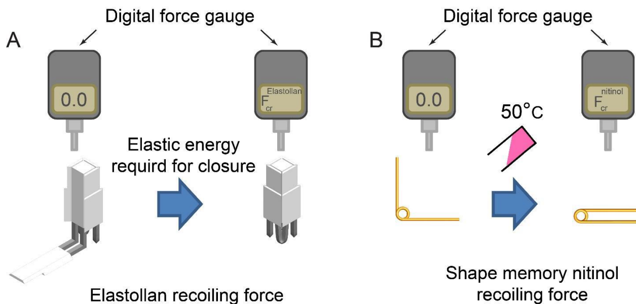
Fig. S6. Mechanical characterization of the flower-like prototype. The recoiling forces were measured using a digital force gauge (FG-3005, Shimpo Instruments) for: (A) the elastomeric recoil elements (Elastollan 1185A), denoted by F_{cr}^{Elastollan} = 0.4\text{ N} , and (B) the shape memory nitinol torsion springs, denoted by F_{cr}^{nitinol} , after triggering by 50°C warm water (colored in pink), with differing number of coils and coil diameters.
