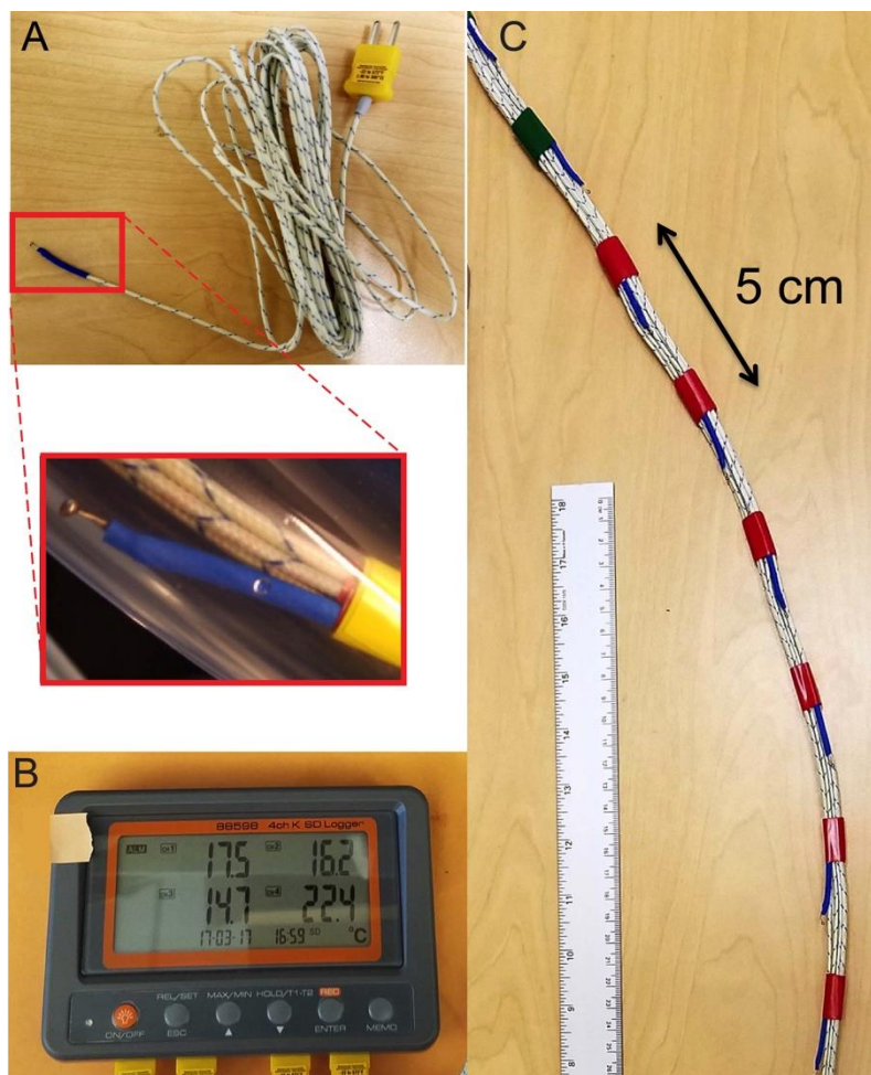
Fig. S1. Temperature testing setup. (A) Bead wire K-type thermocouple. (B) Data logger. (C) Experimental setup consists of 16 thermocouple probes 5 cm spaced.
