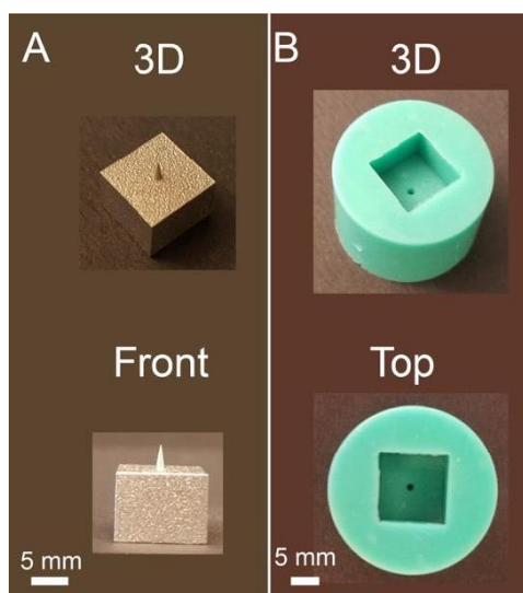
Fig. S7. Fabrication of degradable millineedles. (A) 3D printed metal needle, and (B) negative silicon rubber mold in different views.
