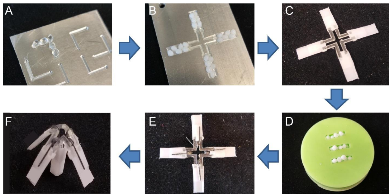
Fig. S4. Fabrication and assembly of the flower-like prototype. (A) Step 1, casting L-shaped beams out of Elastollan 1185A. (B) Step 2, casting PCL arms with the fabricated beams, which results in the strong bond between the arms and beams in (C). (D) Step 3, casting PCL core and drill four holes using 0.6 mm drill bit. (E) Step 4, attaching nitinol torsion springs to arms using an adhesive. (F) Step 5, attaching the torsion springs to the central core and assembling the final flower-like prototype.
