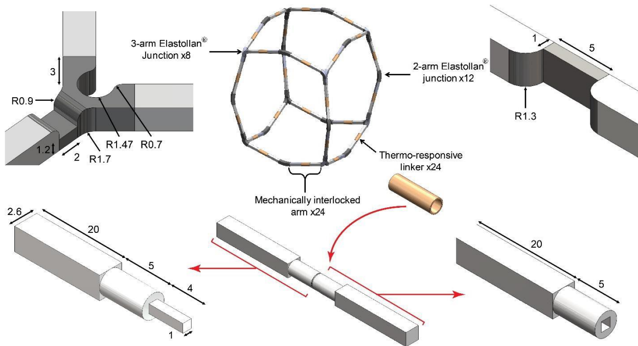
Fig. S8. Reconfigurable mechanical metamaterial as a macrostructure dosage form. CAD model of the macrostructure showing the magnified views of elastic hinges at the corners (3-arm Elastollan junction \times 8 ) and mid-edges (2-arm Elastollan junction \times 12 ), the thermo-responsive linker ( \times 24 ), and interlocking arm-segments (mechanically interlocked arm \times 24 ). All dimensions are in mm.
