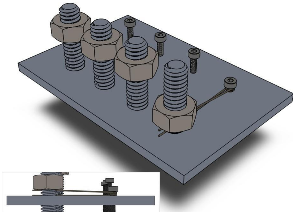
Fig. S5. Heat treatment of shape-memory nitinol. CAD design of the fixture used to immobilize the nitinol wire for shape setting: The fixture is an aluminum plate with 2 mm and 6.35 mm (1/4" – 20) screws across from each other. Each such screw has two small holes drilled approximately 1 thread apart (1.27 mm). A 0.5 mm diameter nitinol wire is threaded through one of the holes in the 6.35 mm screw, which is then tightened until the wire is fixed on one end. The wire is wrapped around the 2 mm screw twice, and then the free end is threaded through the other hole in the 6.35 mm screw. A hex nut is used to fix this end similarly to the previous one. The fixed nitinol is then placed inside the preheated oven at 500°C for 20 minutes and quenched in a room temperature water bath.
