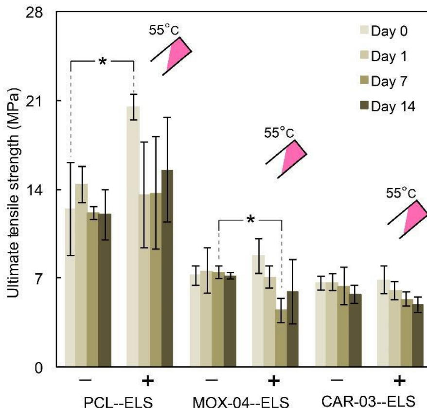
Fig. S11. Mechanical characterization of the interfaces between the polymer arms and elastic hinges by uniaxial tension tests. The ultimate tensile strength of the interfaces between polymer arms (PCL, MOX-4, and CAR-03) and elastic hinges (ELS) after incubation in 37 °C SGF for days 0, 1, 7, and 14. Data reported as mean \pm standard deviation for n = 3 measurements for each group. The tests were performed before (-) and after (+) exposure to 55°C warm water for 20 sec before starting the tension test to investigate the effect of temperature. Two-sample t tests were used to determine the significance. *P < 0.05 [not exposed to warm water (-) versus exposed to warm water (+)].
