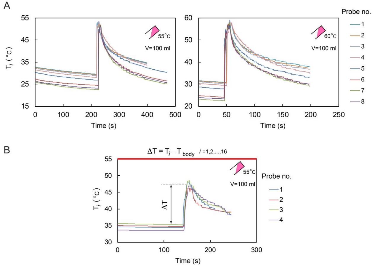
Fig. S2. Evolution of temperature measured while administering warm water. (A) The temperature changes recorded from inserting the setup (8 thermocouple probes) into a 40 cm Tygon Tubing with the same diameter as the esophagus, following pouring of 100 ml of 55 °C and 60 °C. (B) The in vivo temperature changes as a function of time reported for probe numbers n=1,2,3 , and 4 positioned in the upper esophagus of a Yorkshire pig (see Fig. 1A for the position of the probes), upon administrating 100 ml of 55 °C water in 10 seconds.
