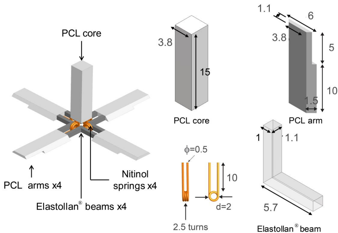
Fig. S3. Flower-like prototype. CAD model of the flower-like prototype made of semi-rigid poly( \epsilon -caprolactone) (PCL) core and arms, shape memory nitinol springs, and elastic Elastollan 1185A beams. All dimensions are in mm.
