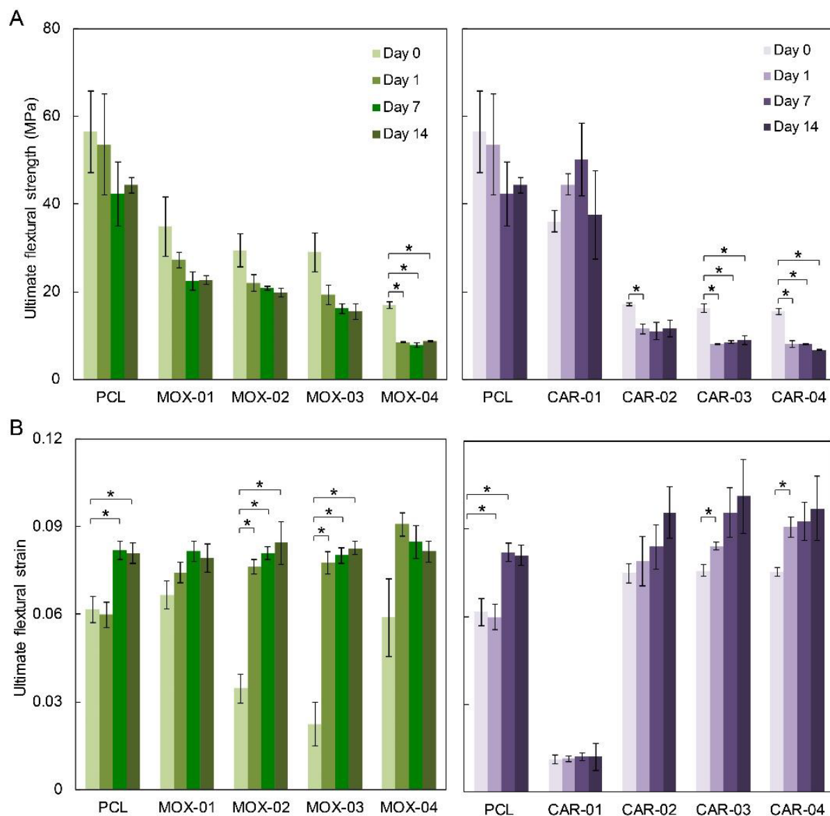
Fig. S10. Mechanical characterization of the drug-loaded arms by three-point bending tests. (A-B) The ultimate flexural strength and strain of drug-polymer arms after incubation in 37 °C SGF for days 0, 1, 7, and 14. The green (moxifloxacin) and purple (carbamazepine) data represent mean \pm standard deviation for n = 3 measurements for each group. * P < 0.05 , one-way ANOVA and post-hoc Bonferroni multiple comparison tests were used to determine the significance (day 1, day 7, and day 14 versus day 0).
