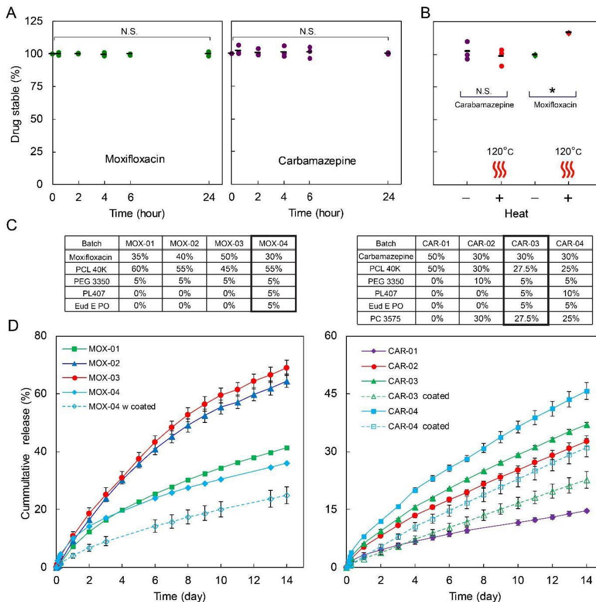
Fig. S9. Drug stability and in vitro release of drug-loaded arms. (A) Moxifloxacin and carbamazepine were incubated in SGF for 24 hours at 37 °C. At various times, drug concentration in SGF was measured using HPLC. Two-sample t tests were used to determine the significance. N.S., not significant (time 0 versus time 24 hours). (B) Stability of the drug upon incubation at 120 °C for 2 hours was assessed using HPLC. Circular markers represent individual data points and dashed lines indicate mean values. Two-sample t tests were used to determine the significance. * P < 0.05 [not heated (-) versus heated (+)]. (C) Summary of different formulations used for in vitro release. MOX-04 and CAR-03 are the selected formulations reported in the main text. (D) In vitro release of the drugs from drug-loaded arms with different formulations incubated in 37 °C SGF for 14 days using HPLC. Solid markers represent the average and error bars represent standard deviation for n = 3 samples in each group.
