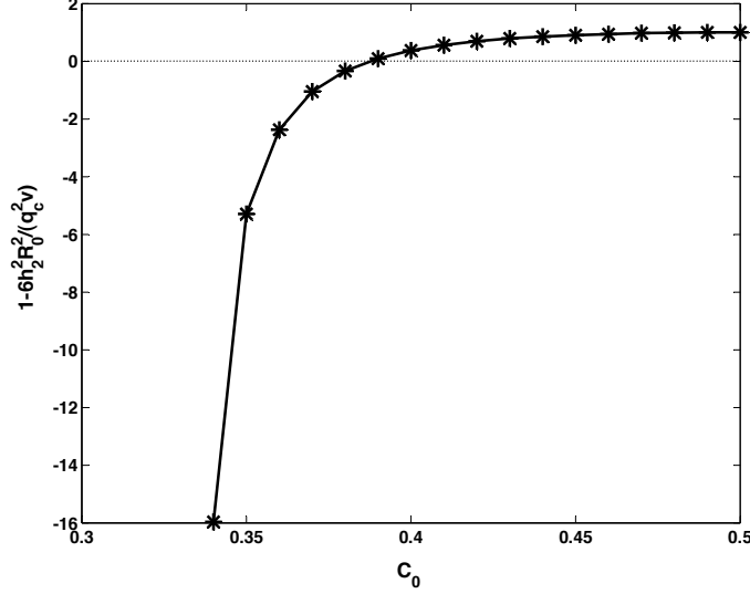
FIG. 11: The values of 1 - \frac{6h_2^2 R_0^2}{q_c^2 v} in the systems where C_0 \in [0.34, 0.50] , Q = 1.6 , and \Omega = 1.6 .
