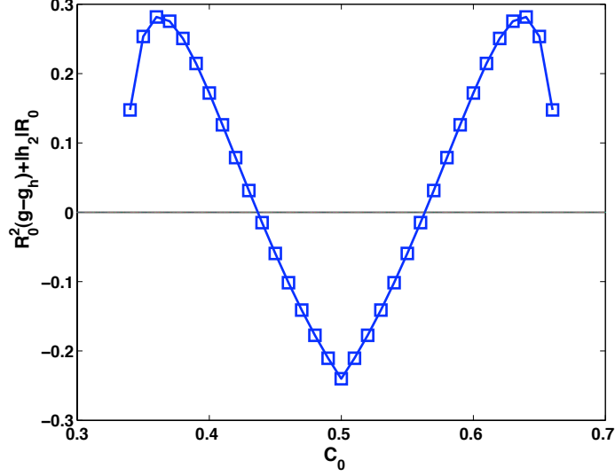
FIG. 9: The growth rate of the most dangerous mode for the perturbations to stripes, obtained using Eqn. (33). The parameters used are Q = 1.6, \Omega = 1.6 , and k = 0 .
