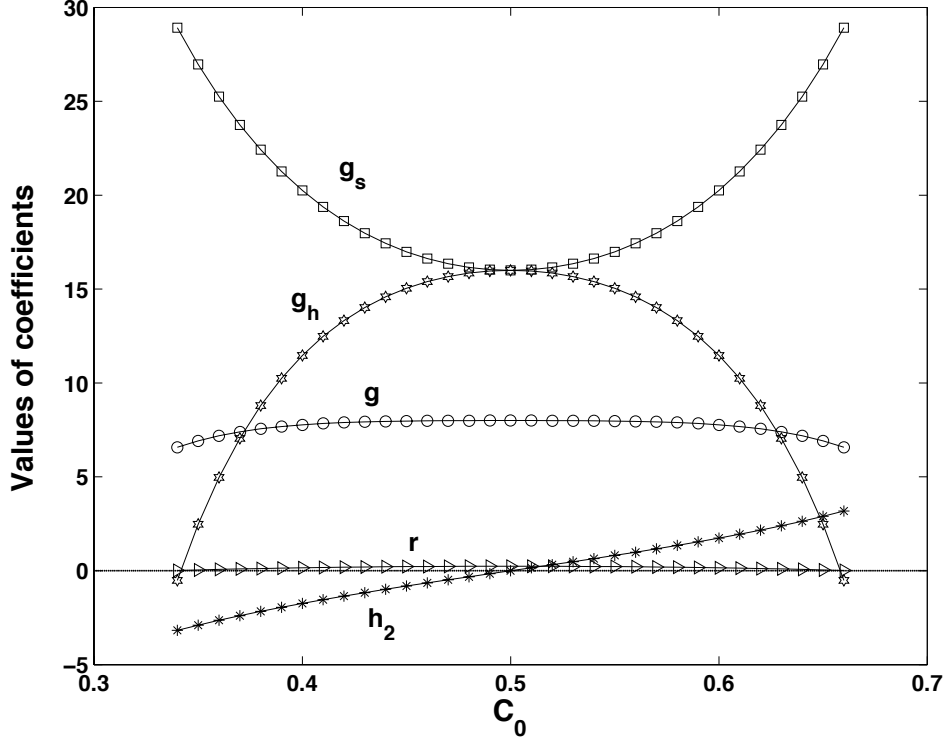
FIG. 4: The values of the coefficients of the Suo-Lu equations at mean concentrations in the range C_0 \in [0.33, 0.67] . The other (fixed) control parameters are Q = 1.6 , and \Omega = 1.6 . The relative ordering of these coefficients determine the stability of patterns at a given set of parameters.
