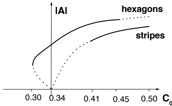
FIG. 10: Bifurcation diagram for the striped and hexagonal patterns in the Suo-Lu model. Stable and unstable solution branches are indicated by solid and dotted lines respectively.
