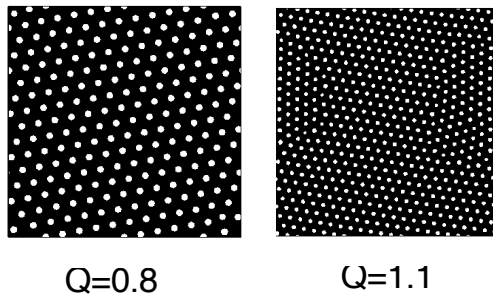
FIG. 2: Patterns at t = 315985 for systems with the same mean concentrations C_0 = 0.31 and \Omega = 2.2 , but with different values of Q . The increase of q where the peak of the dispersion relation is located is reflected in the reduction of the lengthscale in the pattern as Q is increased. The broadening of the band of unstable Fourier modes implies that, typically, the textures are more disordered for large Q . Integrations are implemented on a square domain of 256 \times 256 lattice points with periodic boundary conditions. Each side of the domain is 256l .
