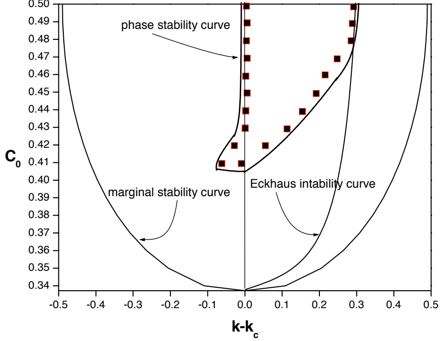
FIG. 7: Numerically computed stability boundaries for striped solutions of Eqn. (4), with parameters Q = 1.6, \Omega = 1.6 . Filled squares show the minimum and maximum wavenumbers of striped arrays that are stable at a given value of C_0 . These results should be compared with theoretical calculations, shown in Fig. 5.
