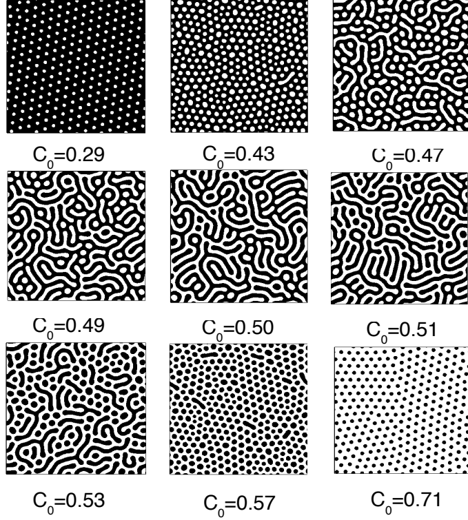
FIG. 3: The patterns at t = 1132234 for systems with 9 different fractional coverages ( Q = 1.0 , and \Omega = 2.2 ). The order in which these patterns appear is the same as that for several experiments on vapor deposition.
