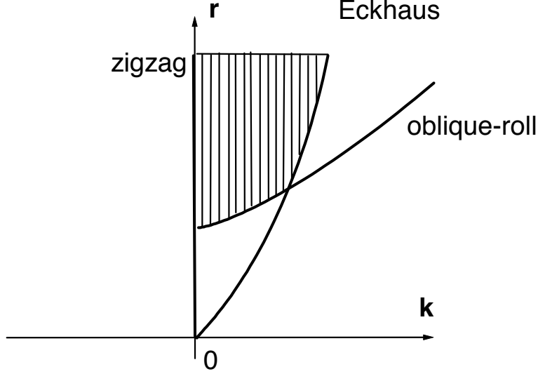
FIG. 5: Stability boundaries of striped patterns for the Suo-Lu model. The hatched region, where striped arrays are stable to small perturbations, is bounded on the left by the zig-zag instability and on the right by the Eckhaus and oblique-roll instabilities. The horizontal line on top is the peak value of r = \Omega + Q^2/4 - 2 (see Eqn. (12)).
