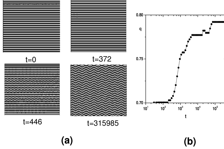
FIG. 6: (a) Snapshots of the spatiotemporal dynamics from an initially striped state ( C_0 = 0.5 , R = 0.01 , q = 0.7 ) under equation (4). The parameters used for the integration are Q = 1.6 , \Omega = 1.6 . The zigzag instability is clearly seen after t \sim 446 . (b) The variation of the mean wavenumber, calculated using disorder function methods, during the evolution.
