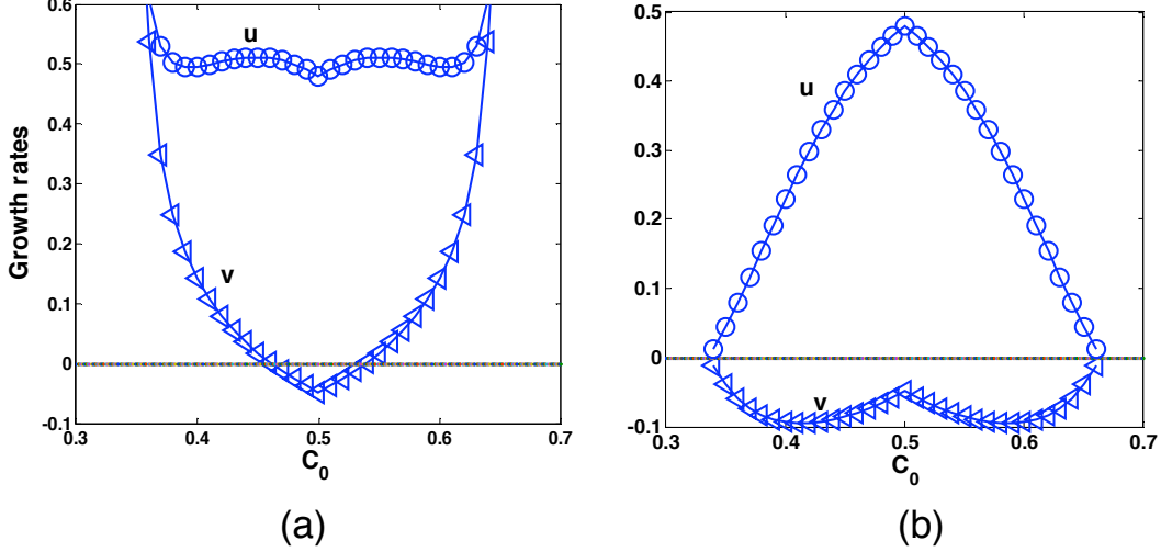
FIG. 8: The growth rates u and v when spatial modulations are ignored: branches with (a) R_0 = R_0^+ and (b) R_0 = R_0^- . The hexagonal state is unstable if either u or v is negative.
