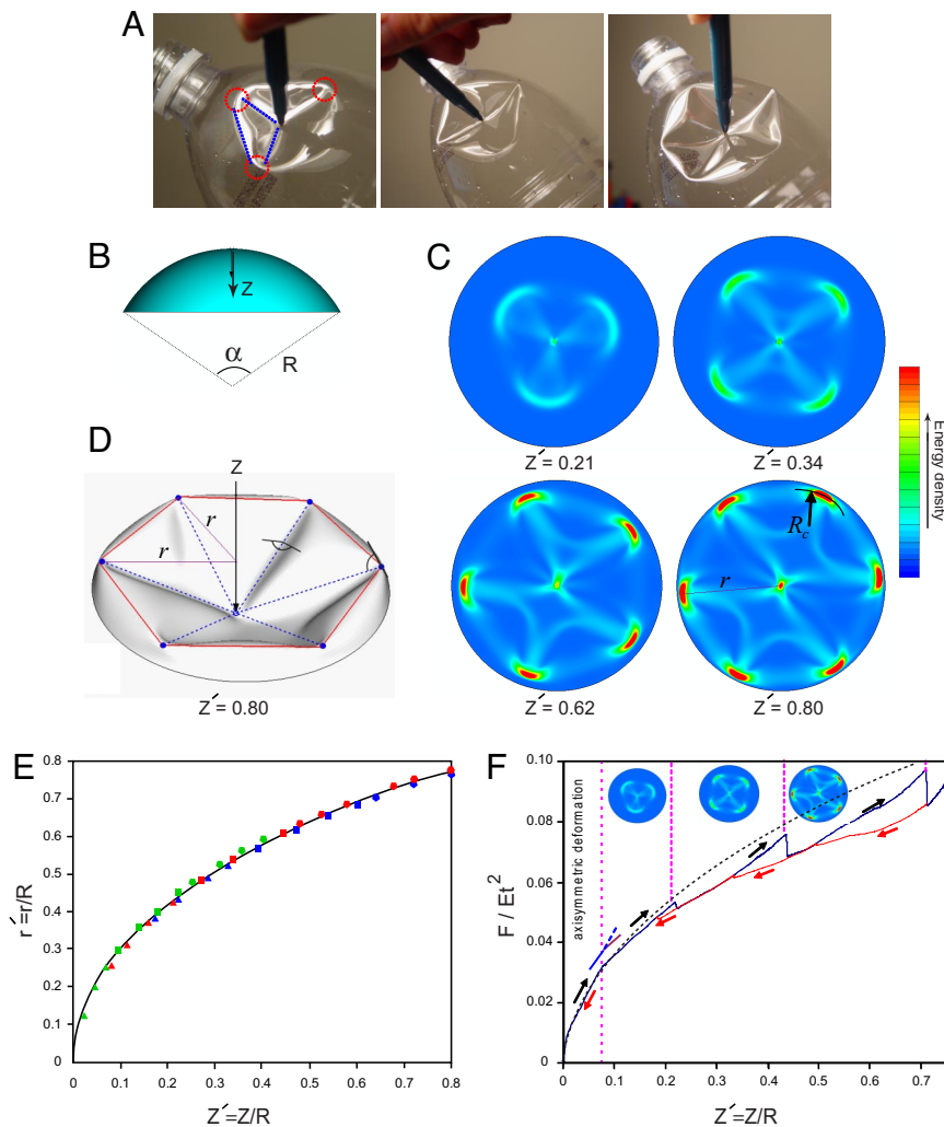
Fig. 1. Indentation of a spherical cap. (A) Localization of deformation in a plastic bottle indented by a sharp pen. The deformation is localized approximately along a polyhedron with a triangular base (Left). As the indentation increases, one of the vertices bifurcates, leading to a polyhedral pattern with a square base (Center). Further indentation leads to further symmetry breaking (Right). (B) Schematic diagram of a clamped spherical cap with natural curvature R , indented at its center. (C) Elastic energy density in the elastic shell ( t/R = 0.005 ) for various normalized indentations Z' (see also Movie S1). The localization of deformation at the vertices is characterized by the localized region of radius R_c (see Fig. S1). (D) Typical deformed configuration of the elastic shell ( t/R = 0.005 for a normalized indentation Z' = Z/R = 0.8 ). The vertices lie approximately on a circle of r'(Z) . (E) The scaled radius r' = r/R , versus the normalized center indentation, Z' . The solid line is given by 5, which for small indentations simplifies to r' \sim \sqrt{Z'} . The results from numerical simulations for different t/R (green: t/R = 0.001 ; red: t/R = 0.005 ; blue: t/R = 0.01 ), where filled triangles, squares, pentagons, and hexagons correspond to deformed configurations with 3, 4, 5, and 6 vertices, respectively. (F) Force-indentation response of an elastic shell with t/R = 0.005 . Localization of deformation, which leads to formation of a pattern with three vertices, occurs at Z' \sim 0.076 . The slopes of the response are shown at this indentation, which indicates \sim 30\% reduction in the apparent stiffness of the elastic shell as the asymmetric buckling pattern emerges, which is consistent with the analytical predictions (17, 18) as well as the approximate solution based on estimating the energy in the rim of the dimple. The dashed line is an approximate solution derived for axisymmetric deformations (14), and it compares qualitatively with the numerical simulations; however, as expected, it overestimates the forces relative to those for the faceted shell. All of the simulations were carried out for a cap with an opening angle \alpha = 120^\circ .
