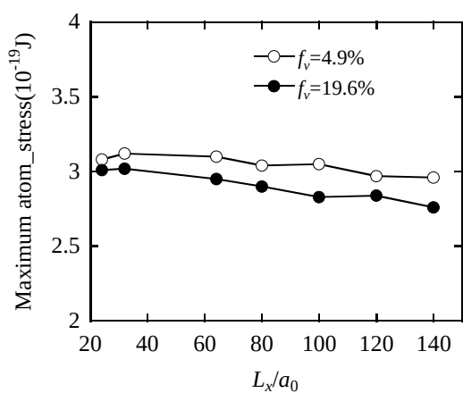
Fig.1 [100]-[010]-[001] crystalline system
