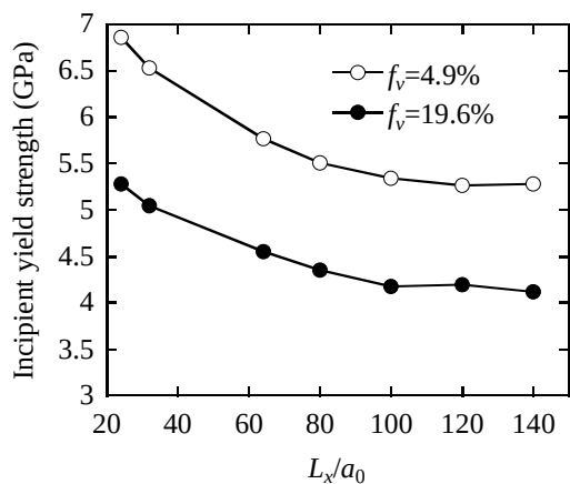
Fig.1 [100]-[010]-[001] crystalline system
