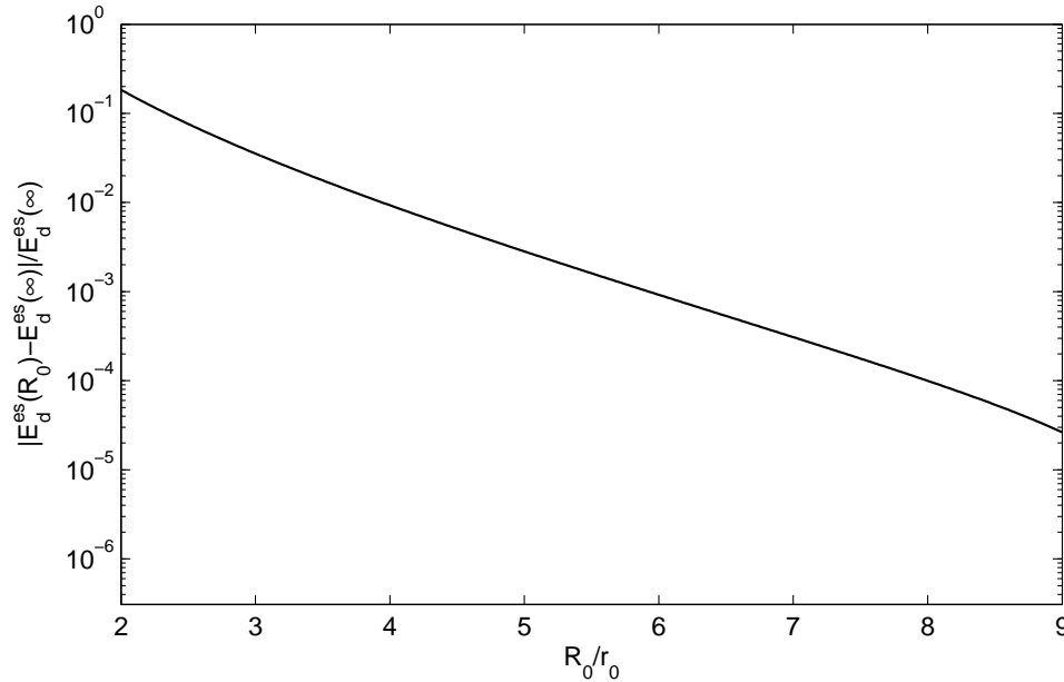
Figure 1: Cell-size effects showing relative error in the electrostatic contribution to the defect energy from finite cell calculations.
