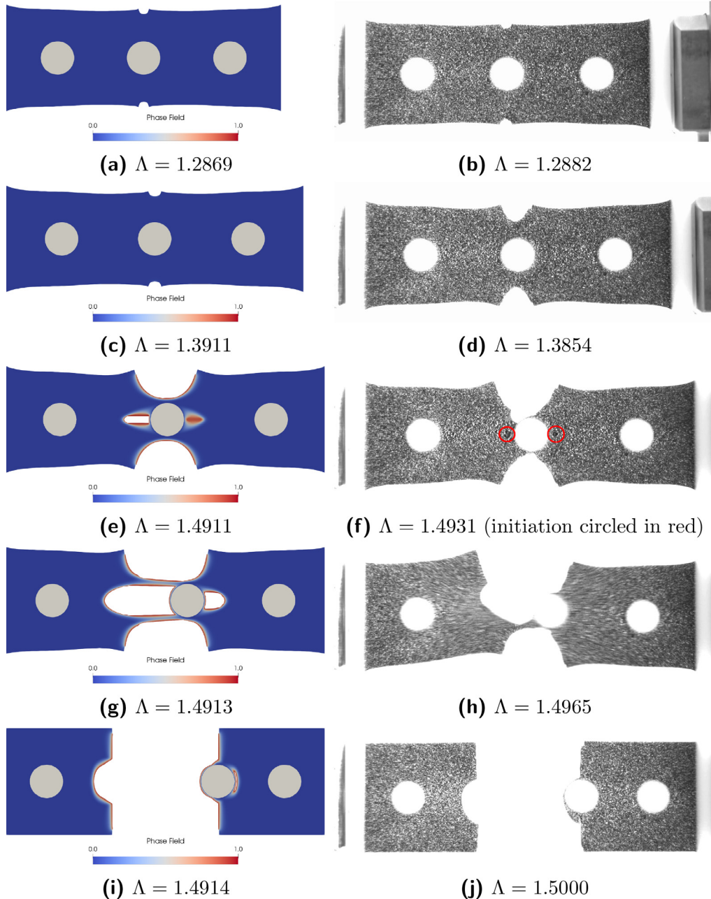
Fig. 7. N05D30 crack initiation sequence at different values of global stretch, \Lambda . Numerical results (left column) and experimental results (right column).
