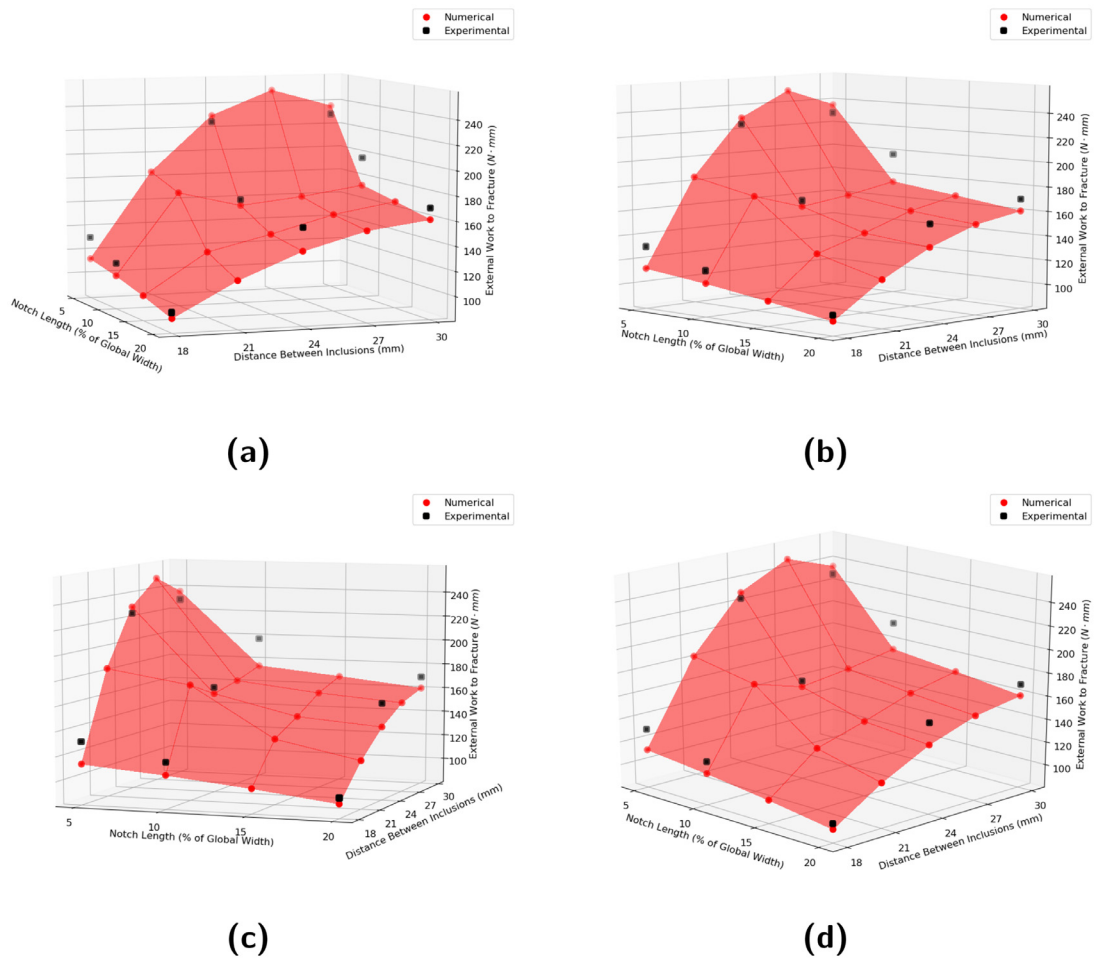
Fig. 15. The numerically computed external work surface viewed from various angles along with the relevant experimentally computed data points.
