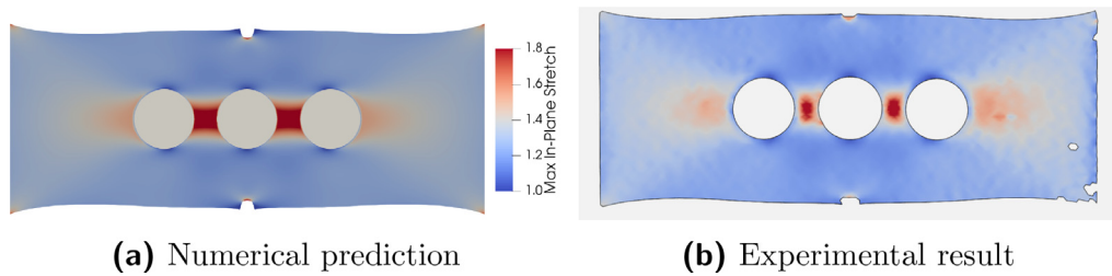
Fig. 6. Stretch comparison for N05D18 at a prescribed end-displacement of 11.8mm compared with DIC image.
