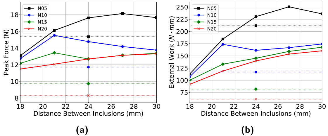
Fig. 14. Numerically predicted (a) peak forces and (b) external work versus distance between inclusions for each notch length. Additionally, a horizontal dotted line (with marker style of the corresponding notch length) signifies the predicted value for the homogeneous case without inclusions. Figure (b) is discussed in the following subsection but placed alongside (a) for ease of comparison.
