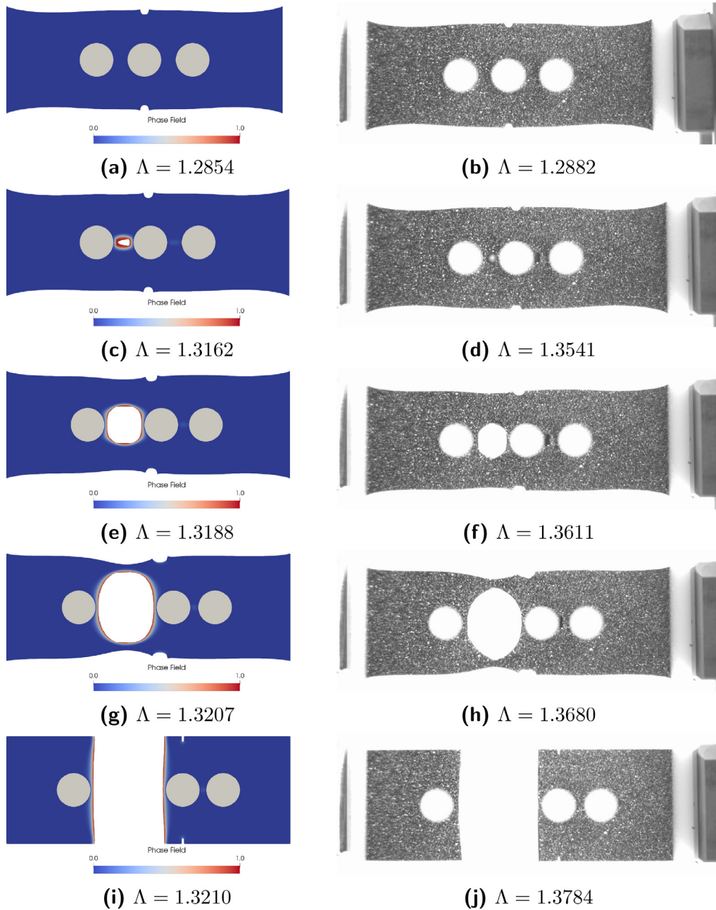
Fig. 11. N05D18 crack initiation sequence at different values of global stretch, \Lambda . Numerical results (left column) and experimental results (right column).
