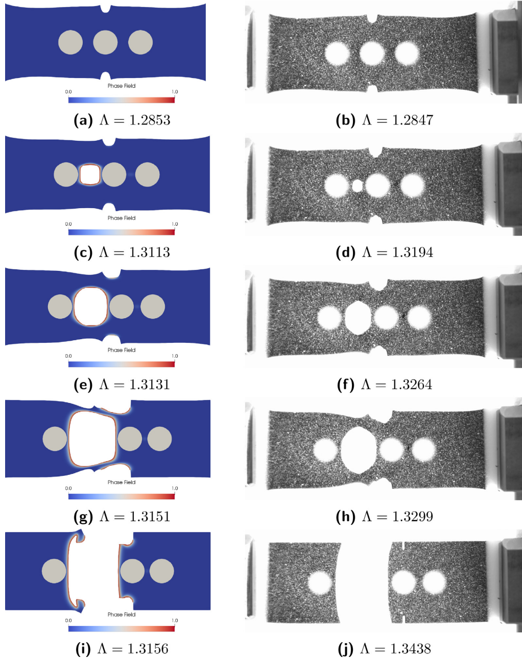
Fig. 10. N10D18 crack initiation sequence at different values of global stretch, \Lambda . Numerical results (left column) and experimental results (right column).
