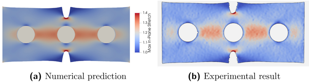
Fig. 5. Stretch comparison for N20D30 at a prescribed end-displacement of 6.6mm compared with DIC image.
