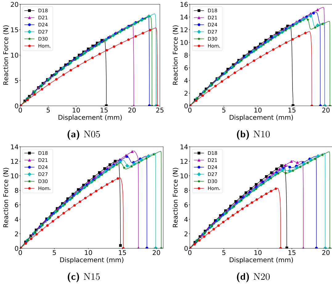
Fig. 13. Numerical force versus displacement curves grouped by notch length along with the numerical prediction for the homogeneous case without inclusions for comparison.
