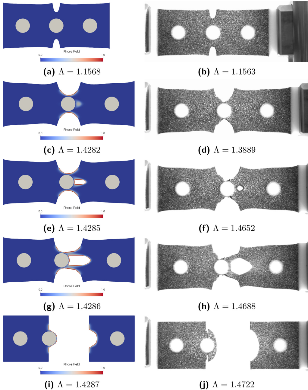
Fig. 8. N20D30 crack initiation sequence at different values of global stretch, \Lambda . Numerical results (left column) and experimental results (right column).
