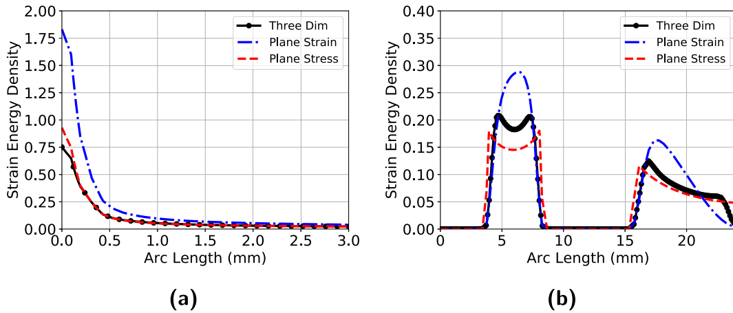
Fig. A.18. Line plots of strain energy density along (a) Line A and (b) Line B as illustrated in Fig. A.17.
