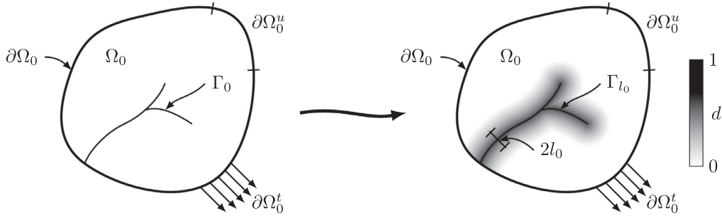
Fig. 1. Phase field approximation of a sharp crack discontinuity in a hyperelastic medium. Note that both figures are drawn in the reference configuration.
