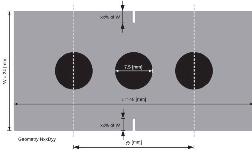
Fig. 2. Geometric parameterization, NxxDyy, in which xx and yy are illustrated graphically.
