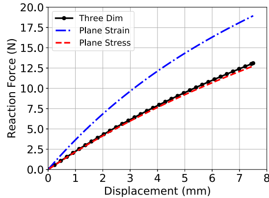
Fig. A.19. Force vs. displacement curves illustrating the consistency of the plane stress approximation with that of the three-dimensional formulation.
