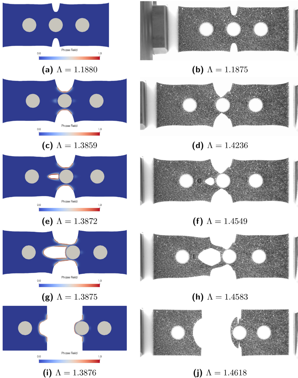
Fig. 9. N20D24 crack initiation sequence at different values of global stretch, \Lambda . Numerical results (left column) and experimental results (right column).
