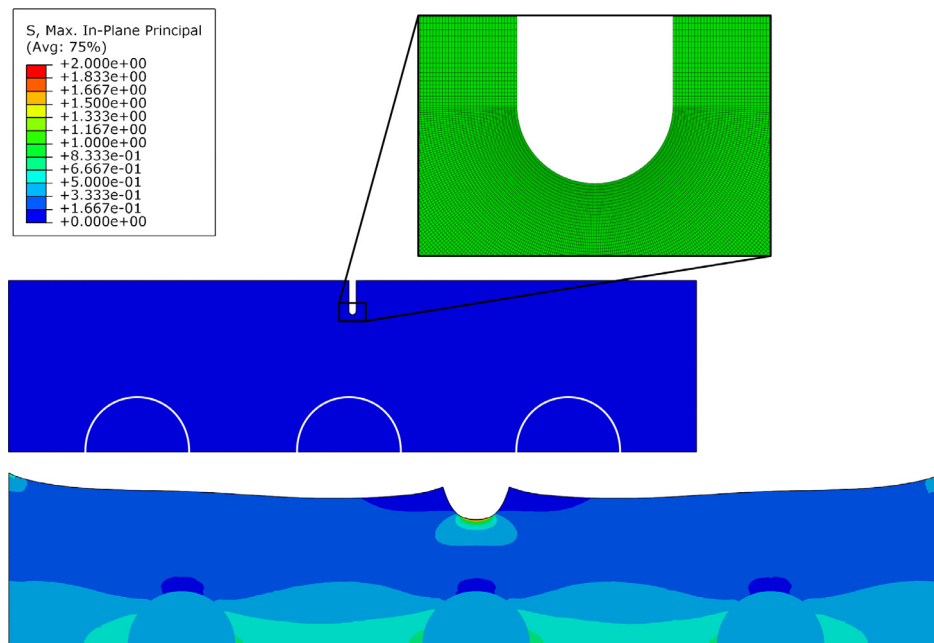
Fig. C.22. ABAQUS result illustration for the N10D30 geometry and notch-tip mesh used for the J-Integral calculation. Note that symmetry along the horizontal plane is employed. Both the undeformed and deformed configurations are presented where the contours illustrate the maximum in-plane principal stress distribution.
