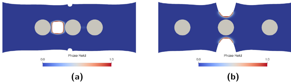
Fig. 4. Predicted crack initiation comparison for (a) N05D18 and (b) N20D30. Note that the plots are clipped at a phase field value of 0.95.
