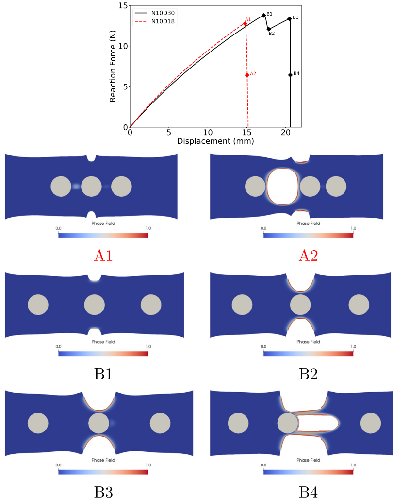
Fig. B.20. (A1 - A2) N10D18 and (B1 - B4) N10D30 numerical snapshots.
