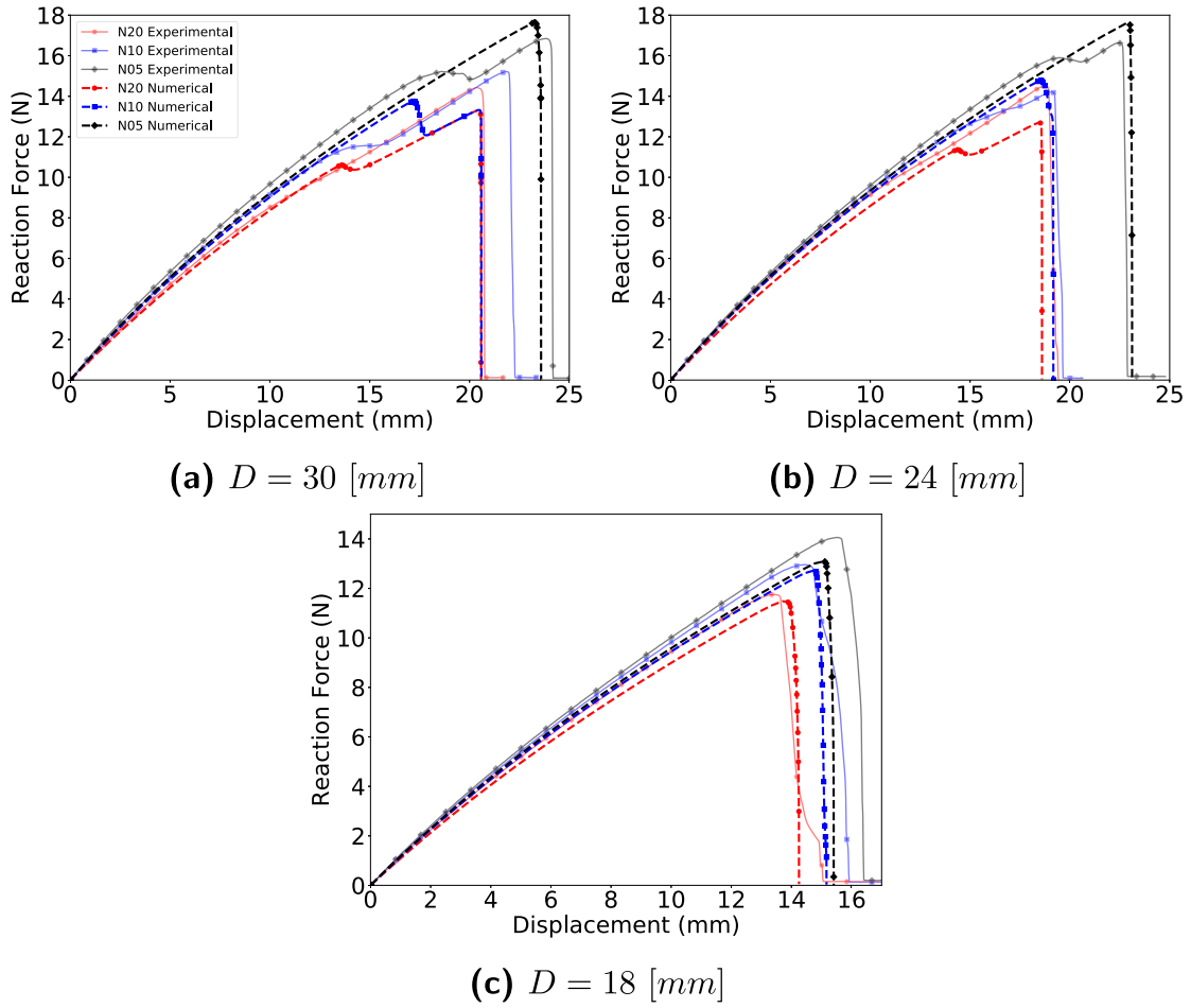
Fig. 12. Experimental and numerical force versus displacement curves grouped by the geometric distance between inclusions ( D ).
