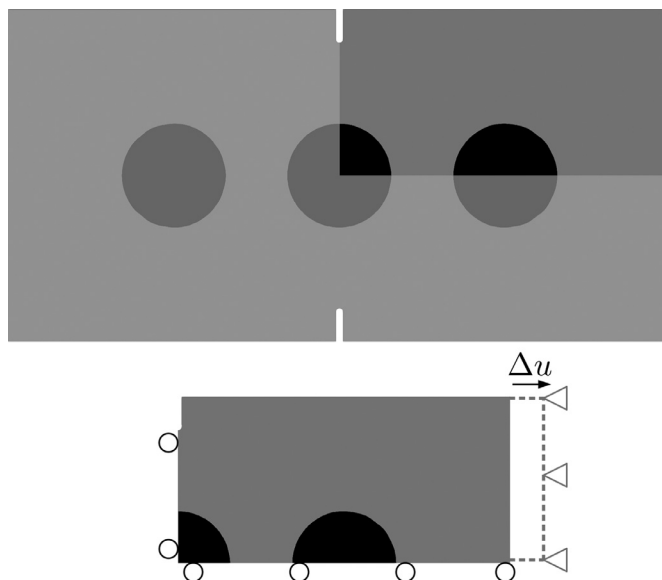
Fig. A.16. Boundary conditions for plane stress validation problem.
