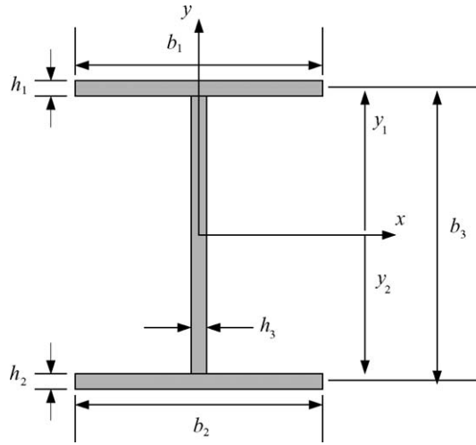
Fig. 2. Geometry of a thin-walled composite open section.
