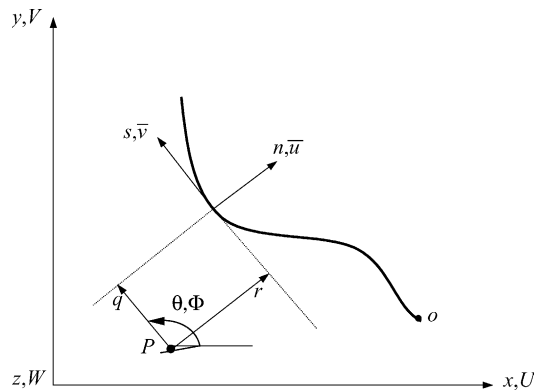
Fig. 1. Definition of coordinates in thin-walled.
