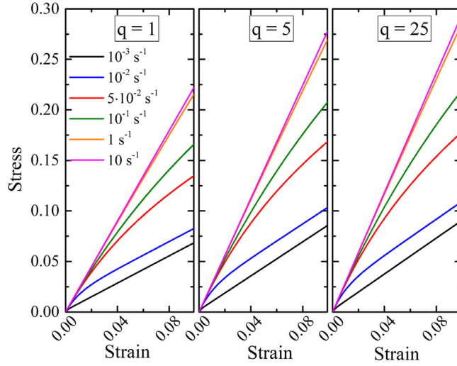
Fig. 6. The modeled stress–strain curves, calculated according (24), for different values of instantaneous compressibility q = \kappa/\mu .
